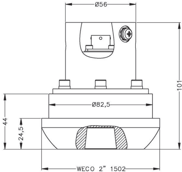
WECO® 2" (1502)
