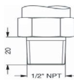
1/2" NPT
