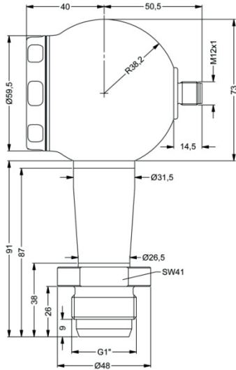
G1" cone
