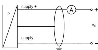
2-wire-system (current)
