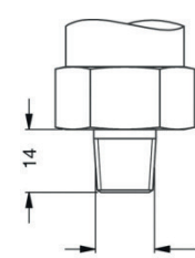
1/4" NPT
