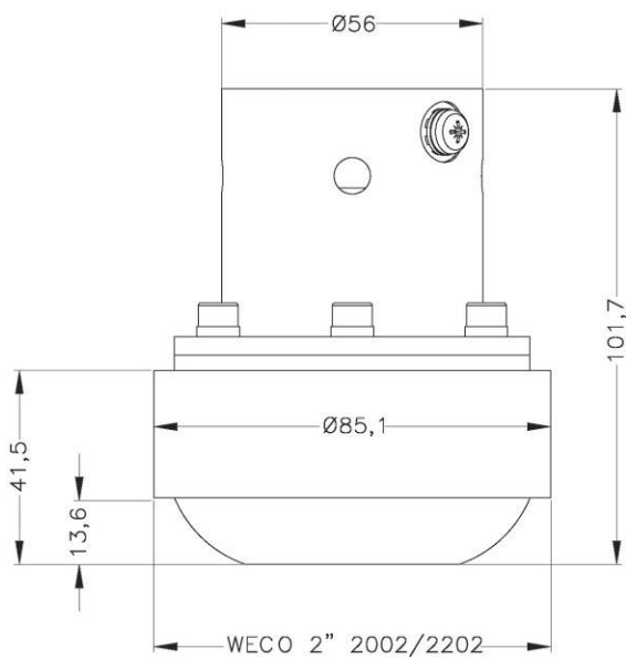
WECO® 2" (2002/2202)
