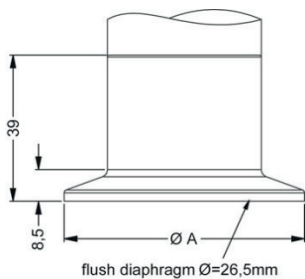
Clamp (DIN 32676)
