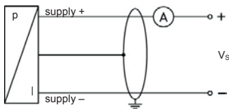
2-wire-system (current)
