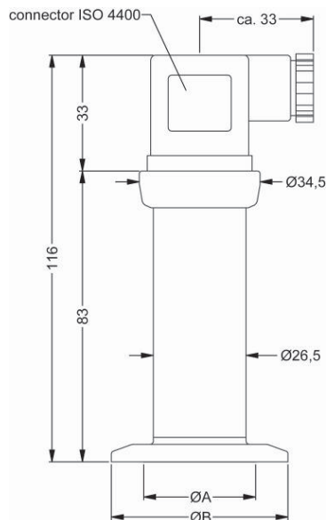
Clamp (DIN 32676)
