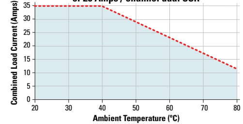
HS201DR w/50 Amps single channel or 25 Amps / channel dual SSR
