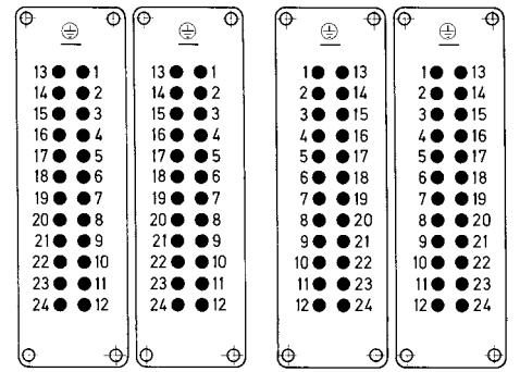
Contact arrangement (view from termination side)
