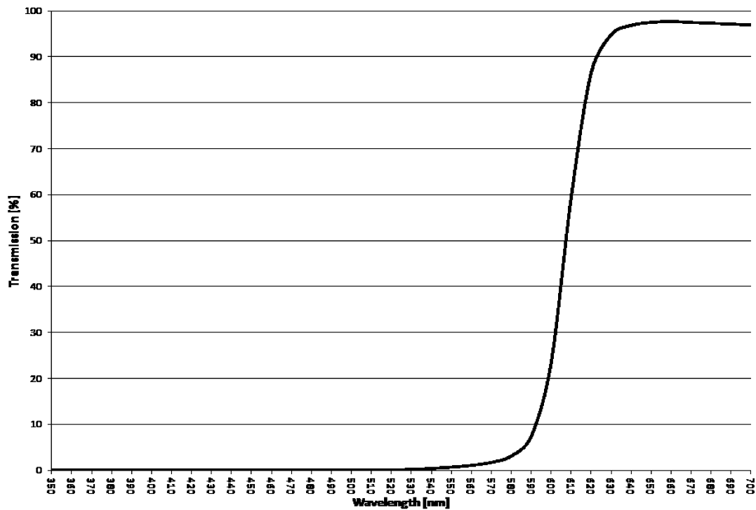
Spectral Transmittance
