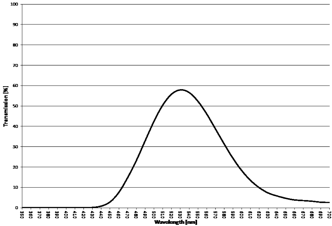
Spectral Transmittance
