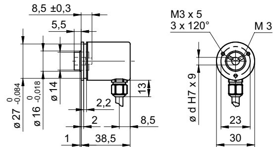
BMSK/BMMK 30 SSI cable radial
