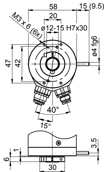
GXP5S - 2 x connector M12, radial
