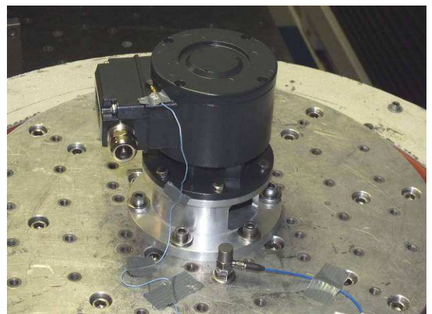
picture 6 Incremental Encoder POG 10 on the vibration table with acceleration sensors during vibration test in Z-axis
