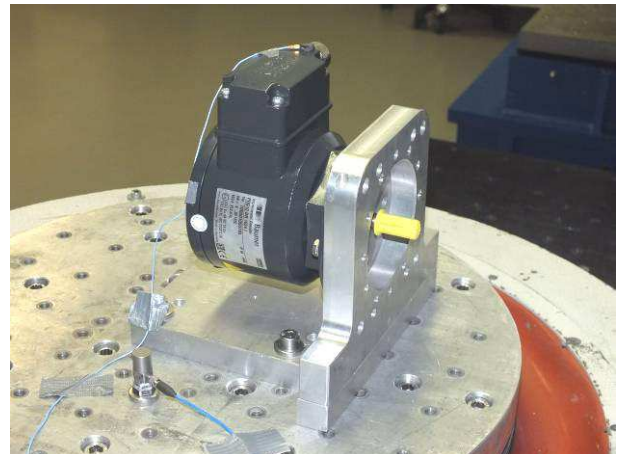
picture 4 Incremental Encoder POG 10 on the vibration table with acceleration sensors during vibration test in Y-axis
