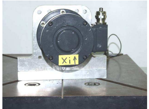
picture 8 Incremental Encoder POG 10 on the shock table with acceleration sensor during and shock test in X-axis, negative direction
