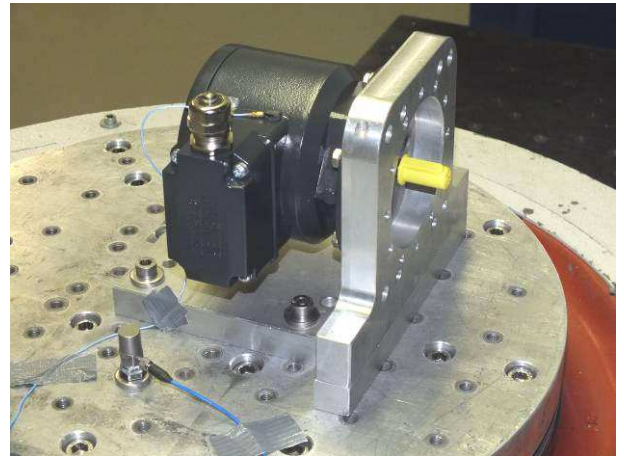
picture 2 Incremental Encoder POG 10 on the vibration table with acceleration sensors during vibration test in X-axis
