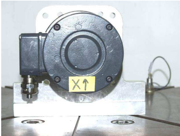
picture 7 Incremental Encoder POG 10 on the shock table with acceleration sensor during shock test in X-axis, positive direction
