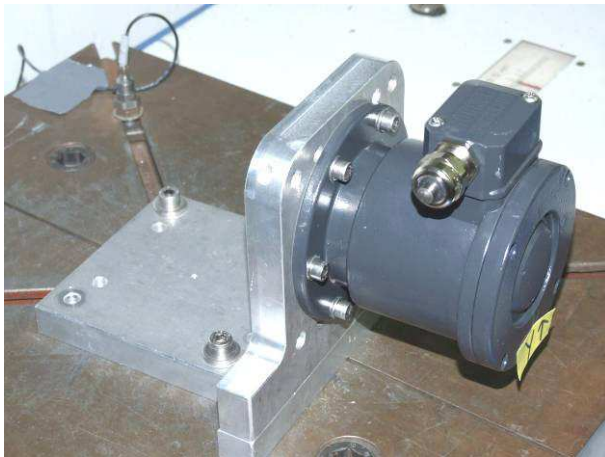
picture 9 Incremental Encoder POG 10 on the shock table with acceleration sensor during shock test in Y-axis, positive direction
