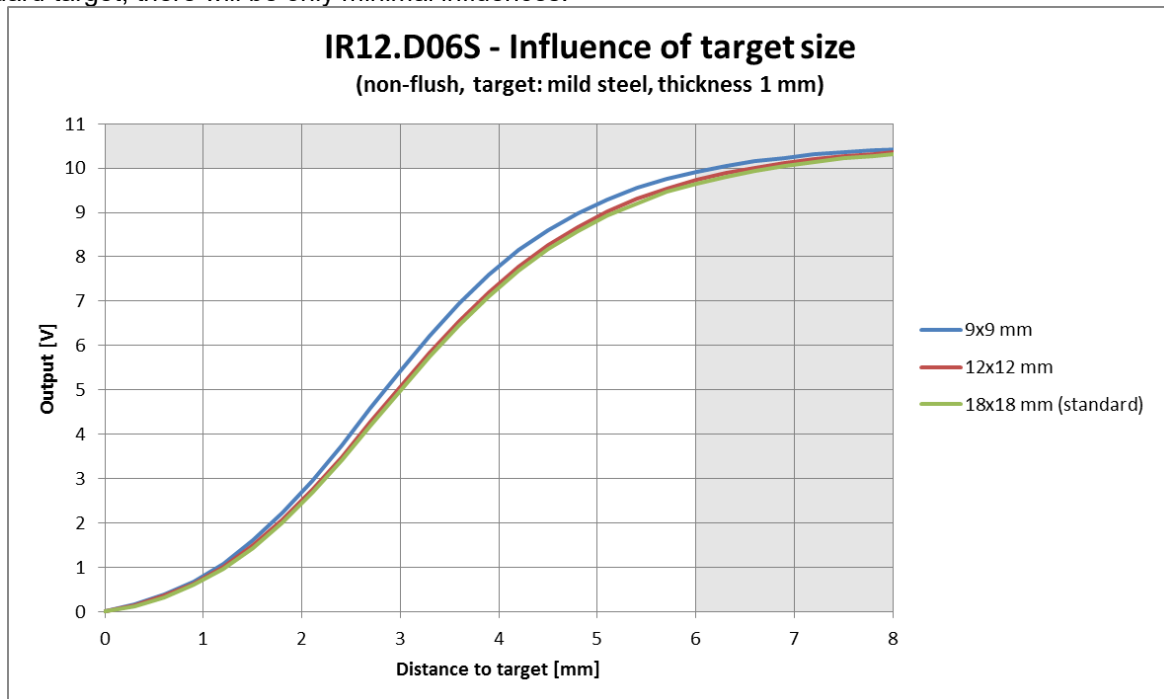
Diagram IR12-D06S sensors: Sensor output (typical values) influenced by targets of different size when the sensor is mounted non-flush.
