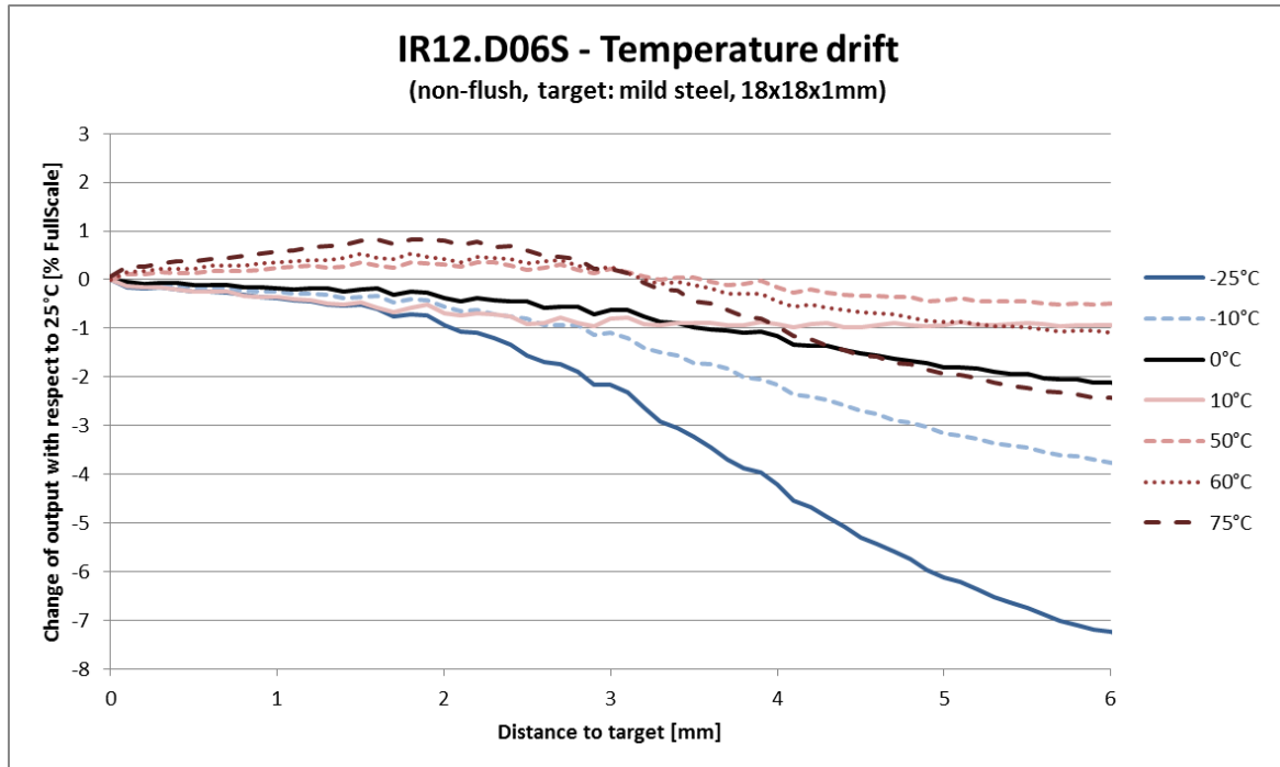
Diagram IR12-D06S sensors: Deviation of the output signal (typical values) at various temperatures and distances relative to the corresponding value at reference temperature (25°C). These sensors show a very small temperature drift for ambient temperatures within 10...60°C.
