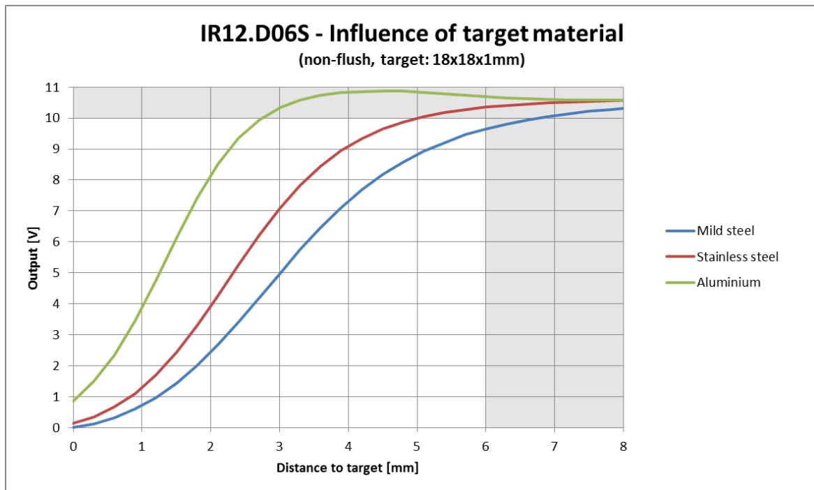
Diagram IR12-D06S sensors: Sensor output (typical values) for different target materials when the sensor is mounted non-flush.
