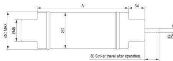
Dimensions - mm
