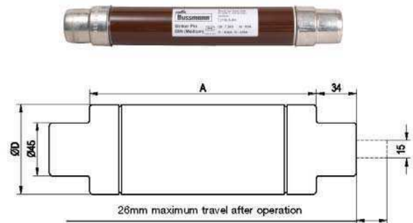
Dimensions - mm
