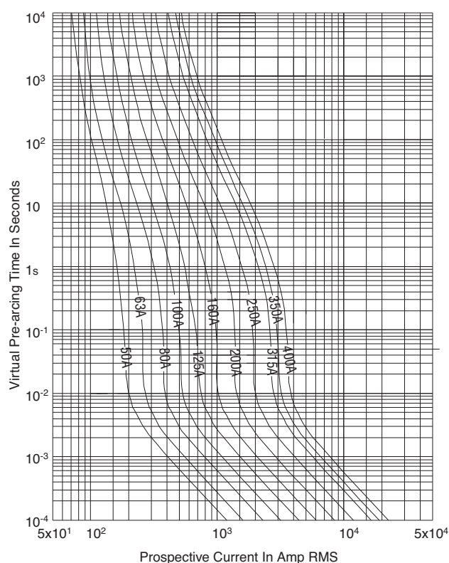
Size 1 — 50-400A: 690V Time-Current Curve
