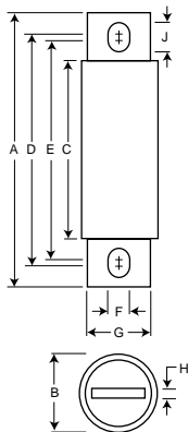
Fig. 1: 5-800 Amp Range
