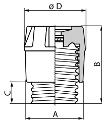
Fuse carrier/cap
