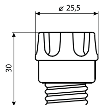
Fuse carrier/cap
