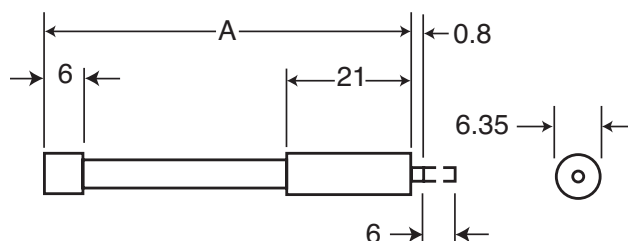
Dimensions - mm
