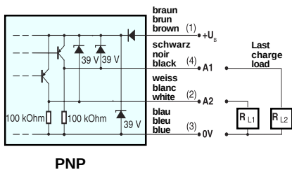
PNP
