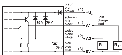
PNP
