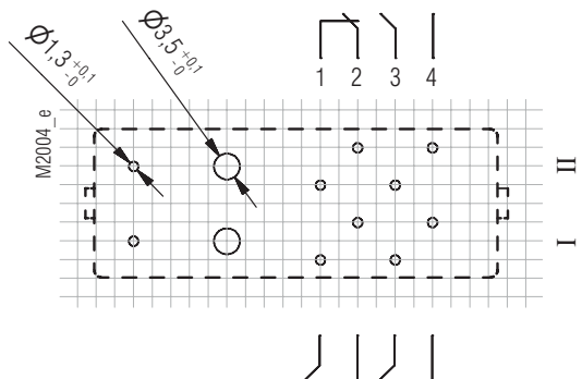
Pin arrangement OA5601.48 3NO/1NC
