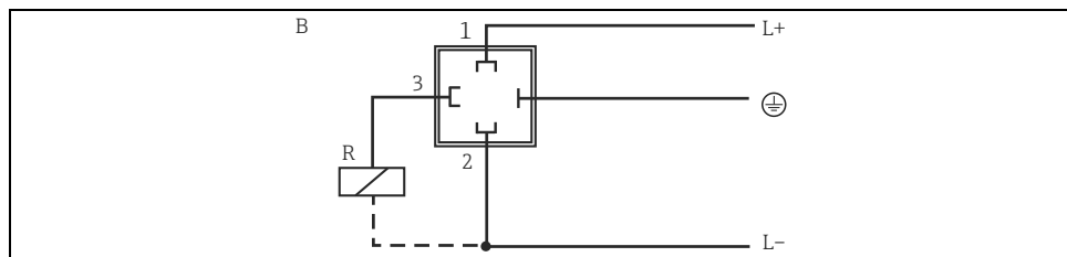
Thermophant T with M 16x1.5 or NPT ½" valve plug
