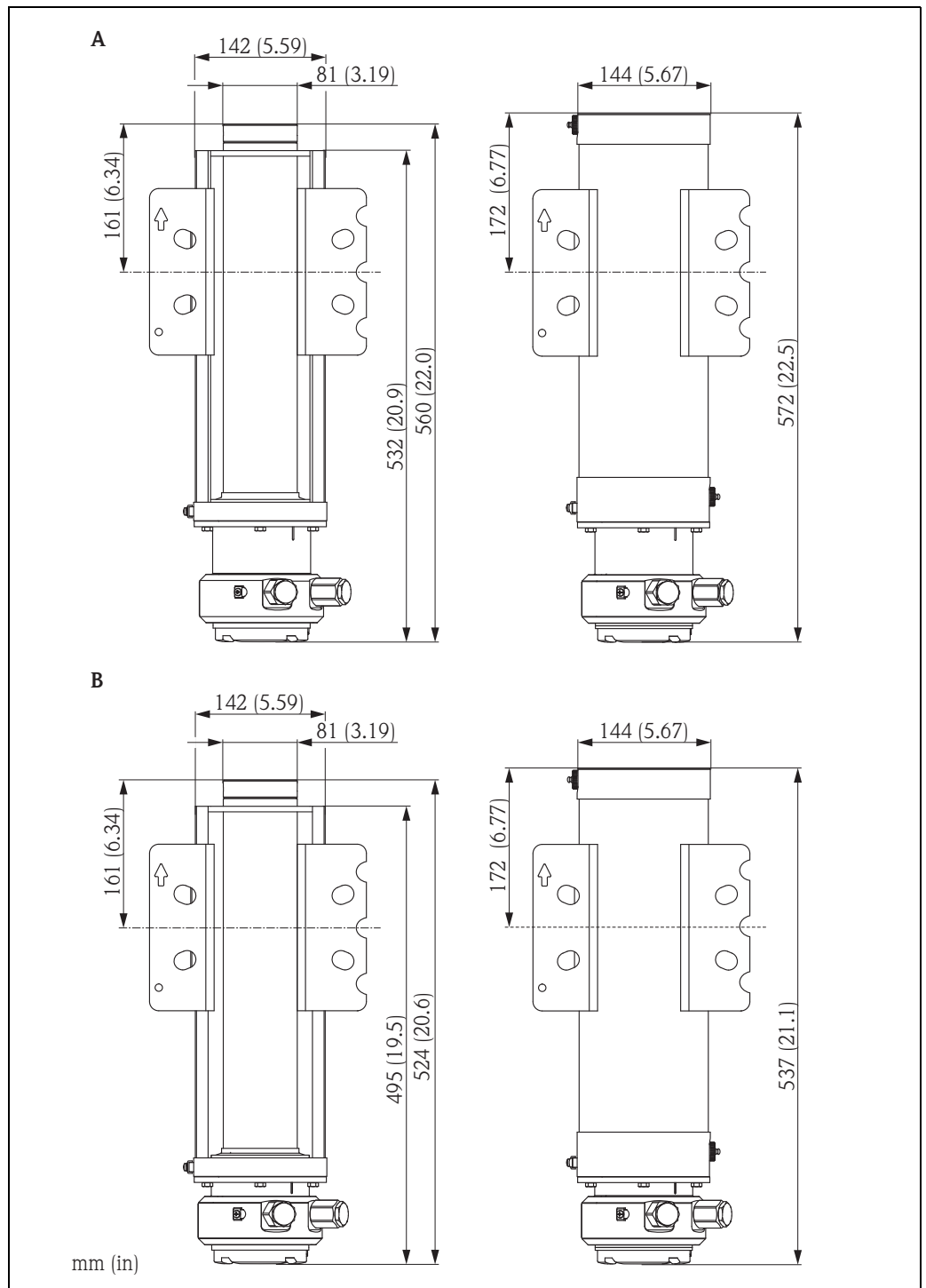
A Ex de - version (left: without water jacket; right: with water jacket) B Ex d, Ex t, non-Ex - version (left: without water jacket; right: with water jacket)
