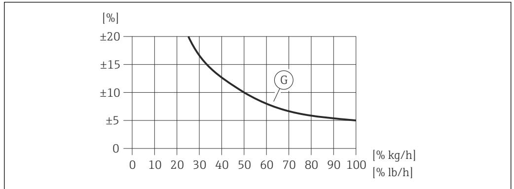
6 Maximum measured error (% mass flow) as % of full scale value. G: Order code for "Calibration flow" (not verified), see the following table
