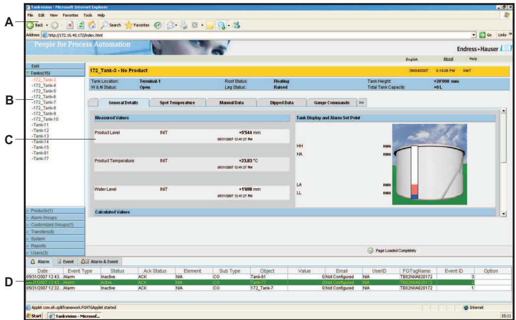
A: Internet Explorer menu and symbol bar; B: Navigation tree; C: Main window; D: Alarms and events viewer
