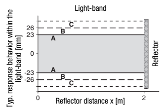
Reference object for detection: 19mm with reflector TKS 100x100
