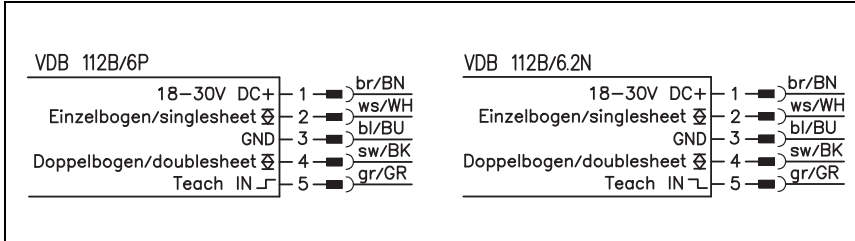
Figure 6.1: Connection diagram VDB 112 B/...
