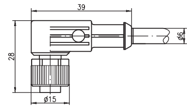
M12 cable angular socket, 3/4/5-pin K-D M12W-...-PVC
