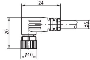
M8 cable angular socket, 3/4-pin K-D M8W-...-PVC
