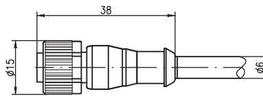
M12 cable axial socket, 3/4/5-pin K-D M12A-...-PVC
