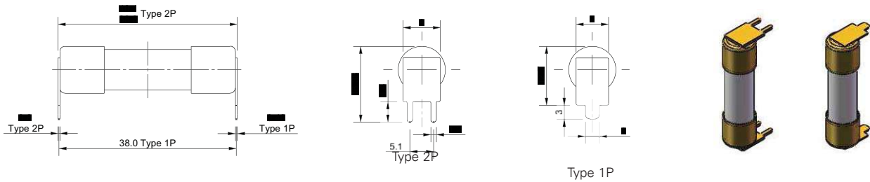
PCB Fixing PV-**A10-1P
