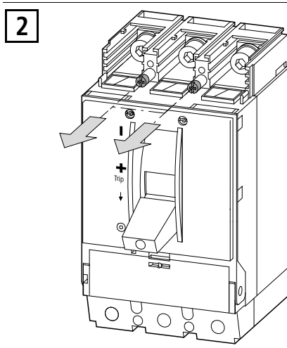
Removal of XKS Screw termination Connectors as shown in the diagrams will enable mounting of XKC pressure Clamp Connector kits.
