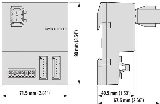
SWD4-FFR-PF1-1
