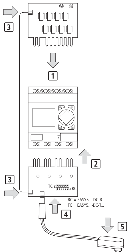
EASY412-DC-SIM: EASY512-DC-...
