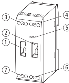
Figure 3: Layout of the SmartWire I/O module
