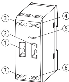
Figure 15: Layout of the SmartWire I/O module
