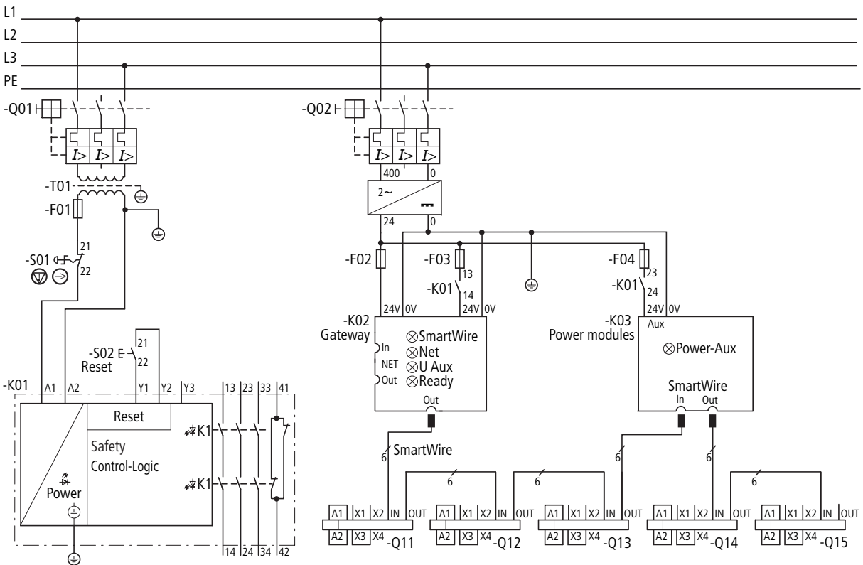
Figure 16: Circuit diagram for safety-relevant switch-offs
