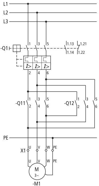
Figure 13: Reversing starter circuit diagram in conjunction with DILM12-XEV
