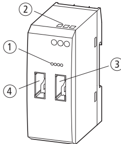
Figure 10: Connecting the SmartWire power module
