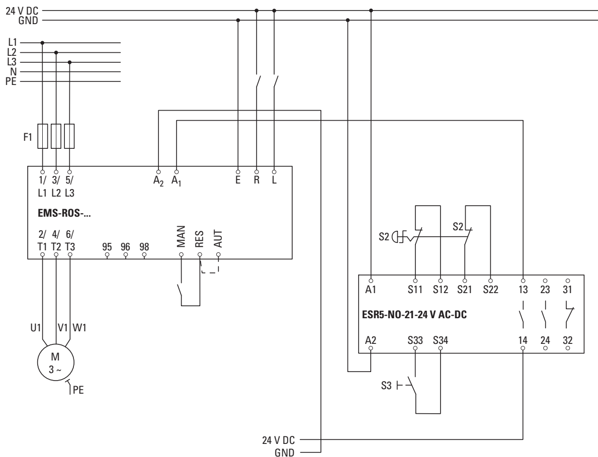
Figure 4: Single-channel main and control current path emergency stop (reduced lifespan) S2 = Emergency stop, S3 = Reset
