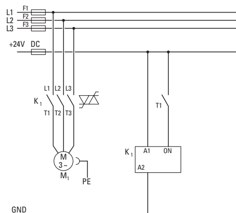
Figure 2: DOL starter
