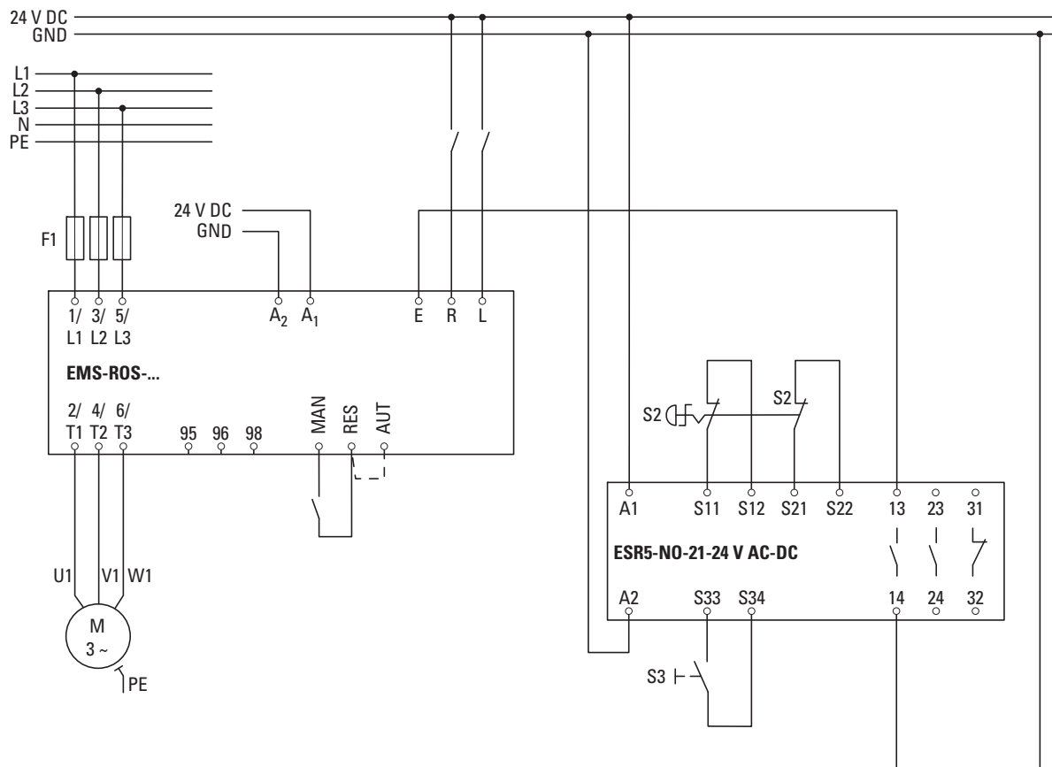
Figure 6: Main and control current path emergency stop (single-channel) S2 = Emergency stop, S3 = Reset
