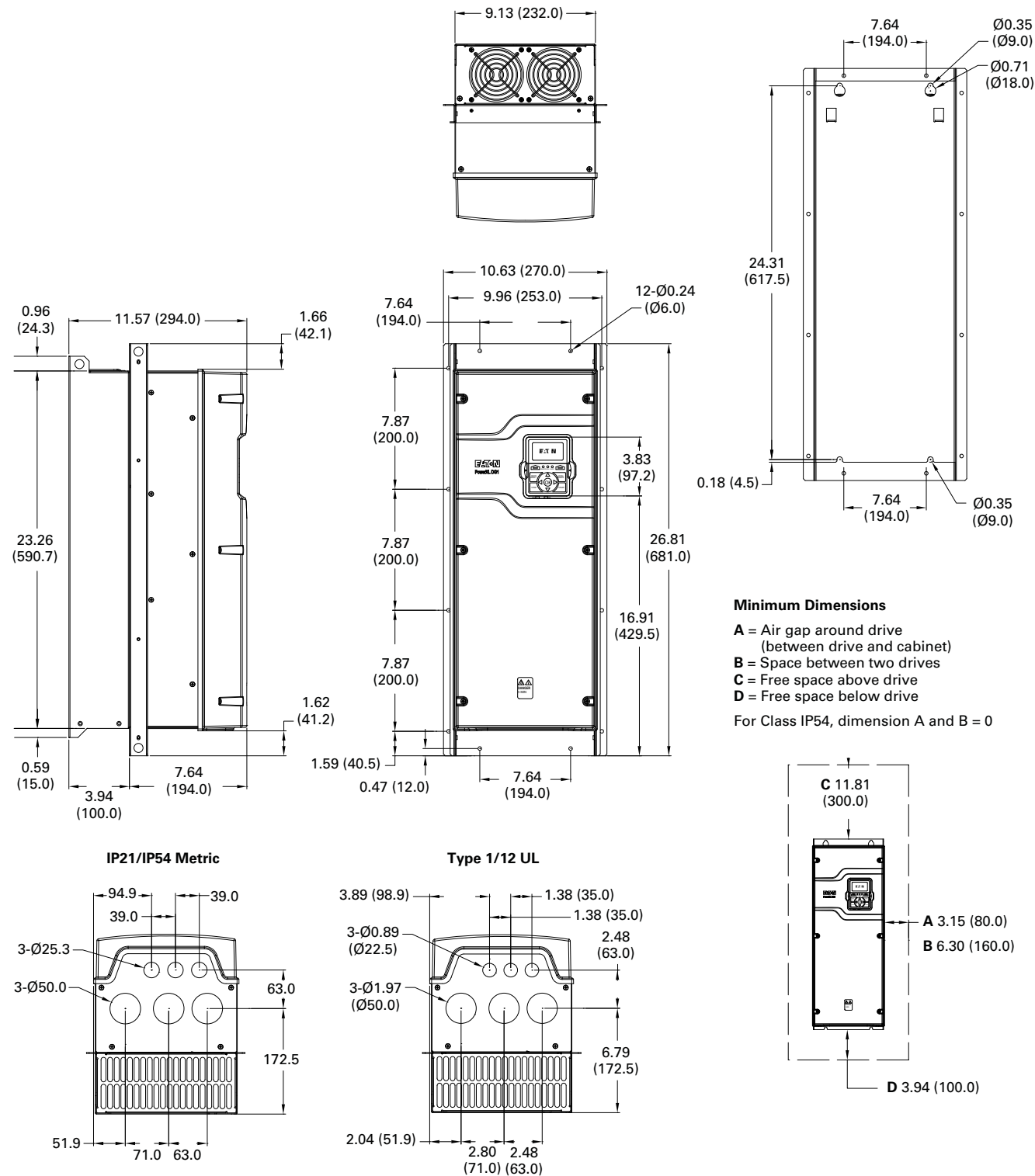
Figure 39. FR4 Dimension Drawing Flange Mount
