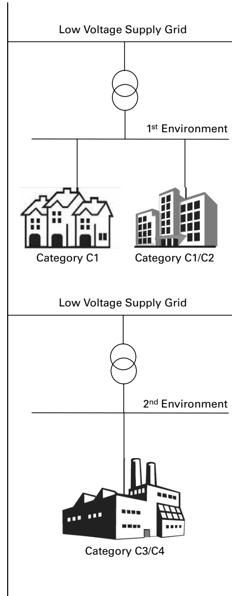
Figure 10. EMC Measures
