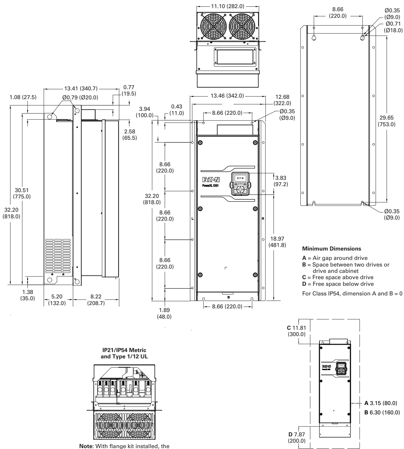
Figure 41. FR5 Dimension Drawing Flange Mount
