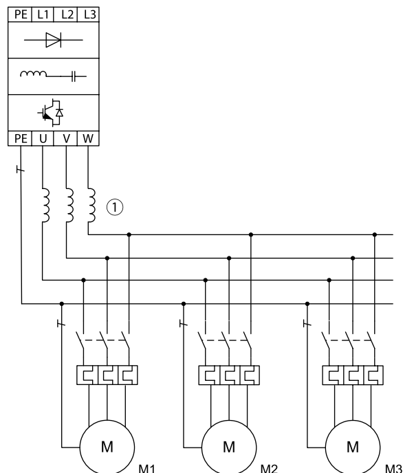
Figure 11. Parallel Connection
