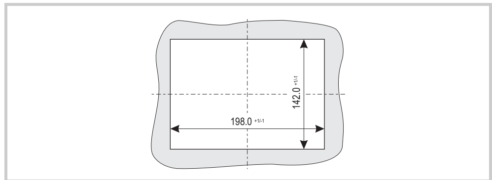
Abb. 25 Mounting cutout for 5.7" devices
