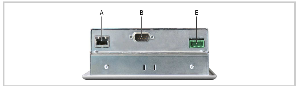
Abb. 9 Interfaces on the connector side of the BAS, CAN and MPI devices (figure shows CAN device)
