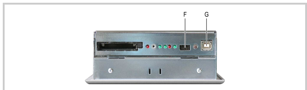
Abb. 11 Interfaces on the service side of the BAS, CAN and MPI devices (figure shows service side of BAS, CAN and MPI devices)
