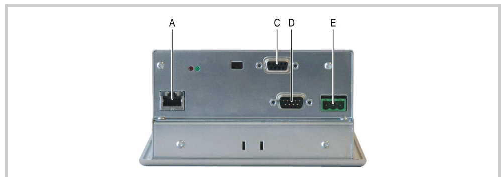
Abb. 10 Interfaces on the connector side of the SKS devices
