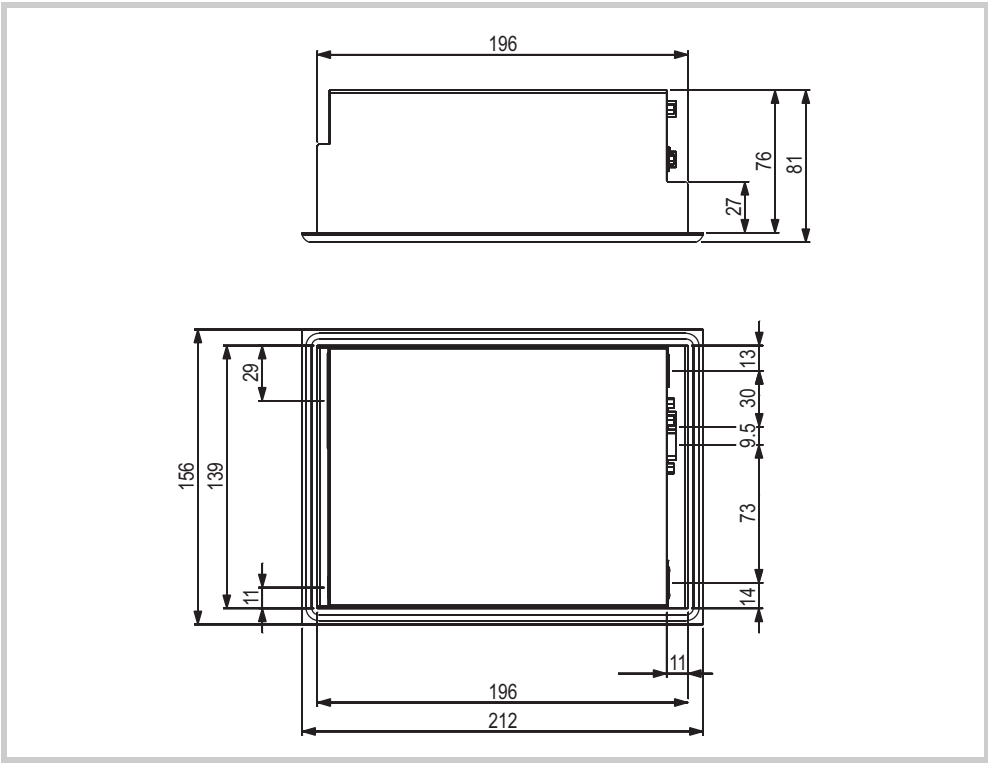
Abb. 33 Mechanical dimensions of the SKS devices in mm
