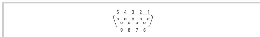
Abb. 21 Profibus interface (9-pin, D-Sub, female, UNC)
