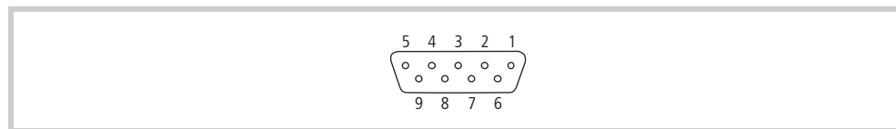
Abb. 23 RS485 interface (9-pin, D-Sub, female, UNC)
