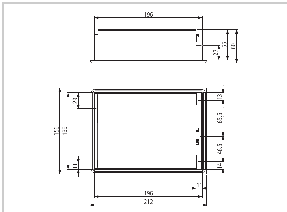
Abb. 32 Mechanical dimensions of the BAS, CAN and MPI devices in mm
