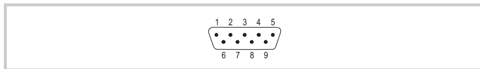
Abb. 19 CAN interface (9-pin, D-Sub, male, UNC)
