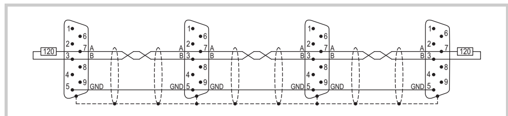
Abb. 24 Bus segment with four bus stations
