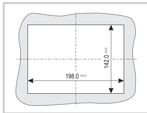
Abb. 23 Mounting cutout for 5.7" devices
