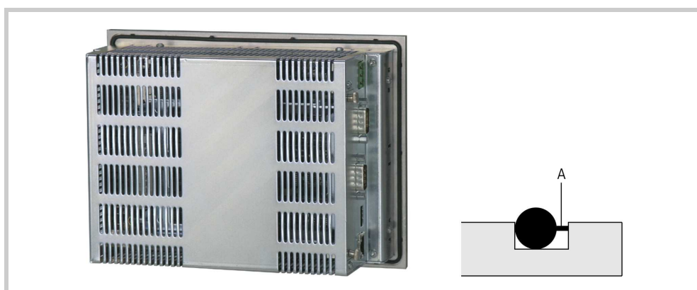
Abb. 40 Seal fitted (detail shows optimum position of a securing tab (A))
