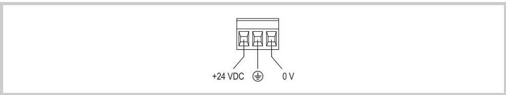
Abb. 15 Phoenix Contact MSTB 2.5/3-ST-5.08 connector (view from the wiring side)
