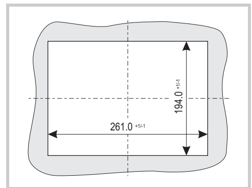
Abb. 24 Mounting cutout for 8.4" devices
