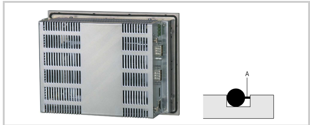
Abb. 34 Seal fitted (detail shows optimum position of a securing tab (A))
