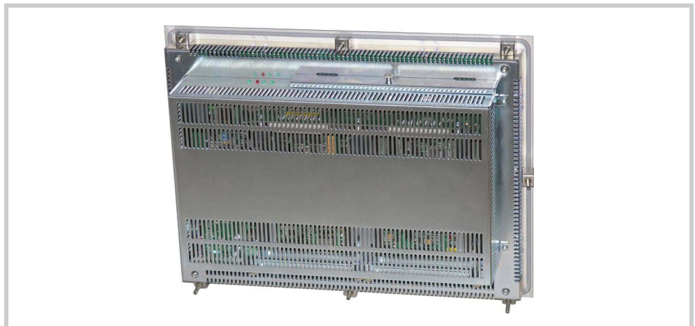
Abb. 28 10.4" and 12.1" devices with eight retaining brackets (meet IP65 requirements)
