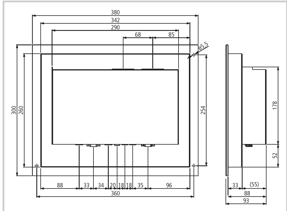
Abb. 50 Mechanical dimensions of the 12.1" devices with 4-hole front in mm
