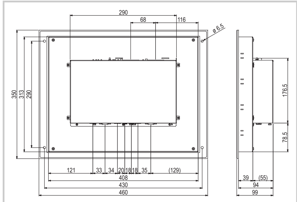
Abb. 52 Mechanical dimensions of the 15" devices with 4-hole front in mm
