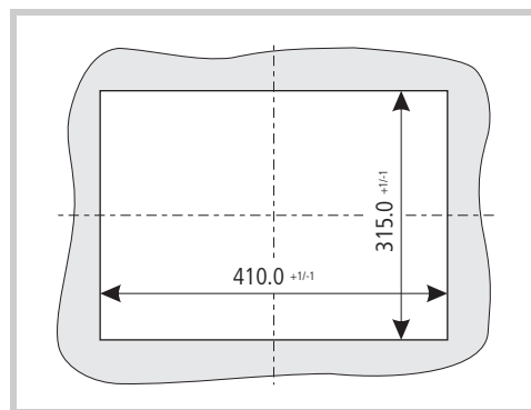
Abb. 24 Mounting cutout for 15" devices
