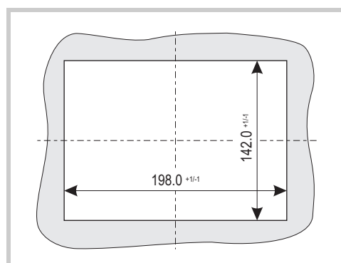
Abb. 20 Mounting cutout for 5.7" devices
