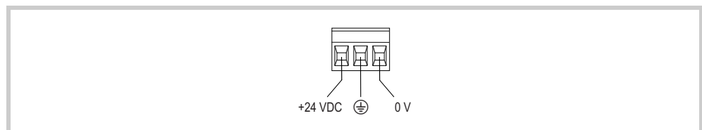
Abb. 13 Phoenix Contact MSTB 2.5/3-ST-5.08 connector (view from the wiring side)
