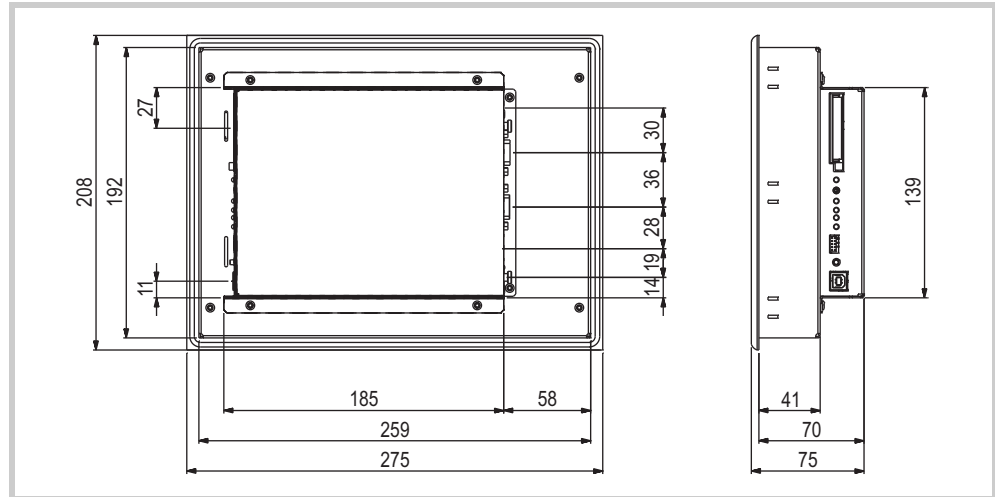
Abb. 29 Mechanical dimensions of the 8.4" devices in mm
