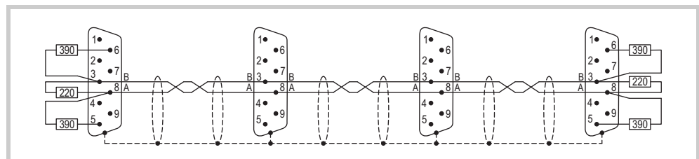
Abb. 19 Bus segment with four bus stations
