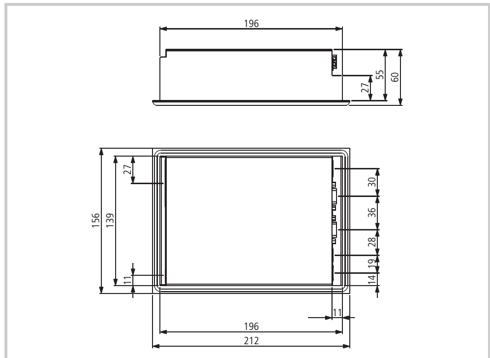
Abb. 28 Mechanical dimensions of the 5.7" devices in mm
