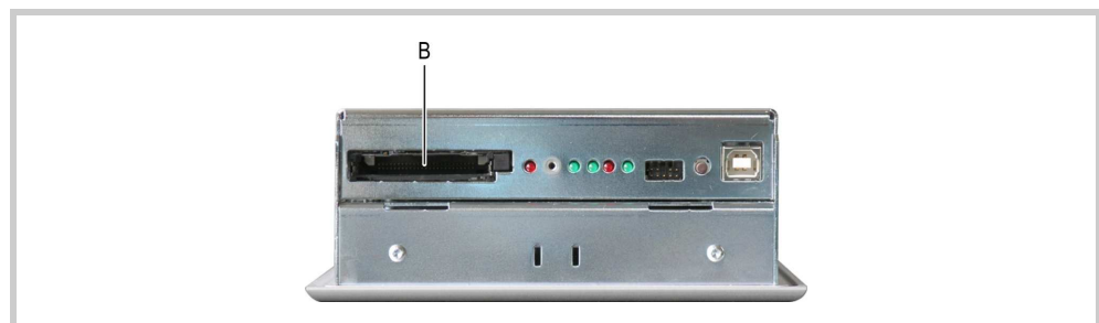
Abb. 27 Service side of the device (CF slot cover removed)
