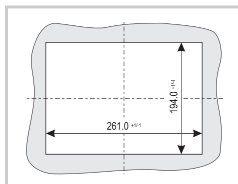
Abb. 21 Mounting cutout for 8.4" devices
