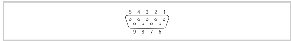
Abb. 18 Profibus interface (9-pin, D-Sub, female, UNC)
