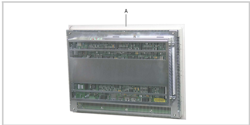
Abb. 22 Groove for sealing strip (A)
