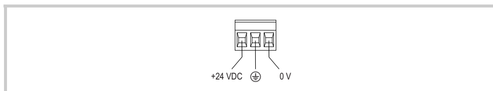
Abb. 12 Phoenix Contact MSTB 2.5/3-ST-5.08 connector (view from the wiring side)
