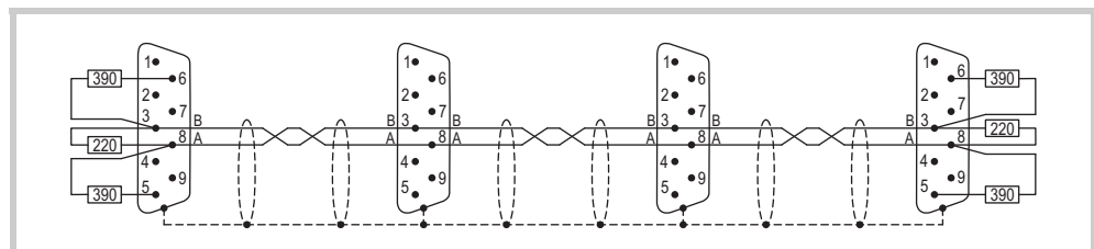
Abb. 18 Bus segment with four bus stations
