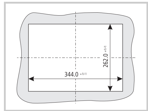
Abb. 20 Mounting cutout for 12.1" devices
