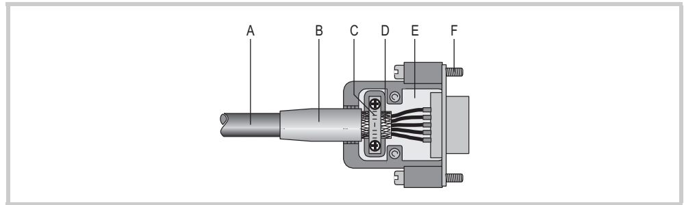
Abb. 10 Cable prepared with D-Sub connector
