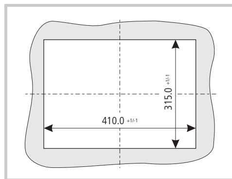
Abb. 21 Mounting cutout for 15" devices
