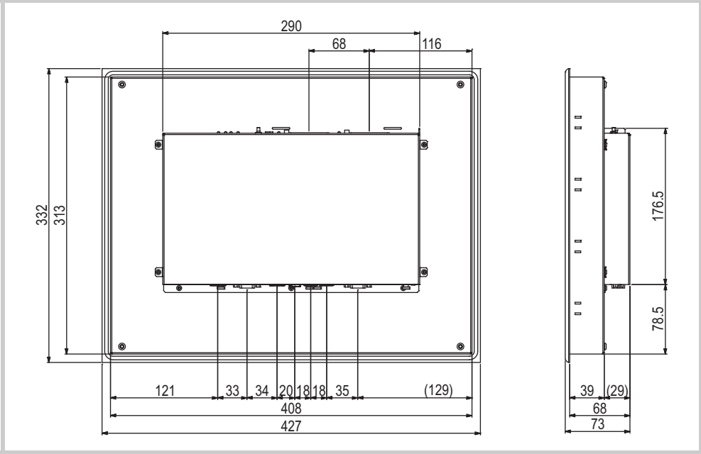
Abb. 32 Mechanical dimensions of the 15" devices in mm
