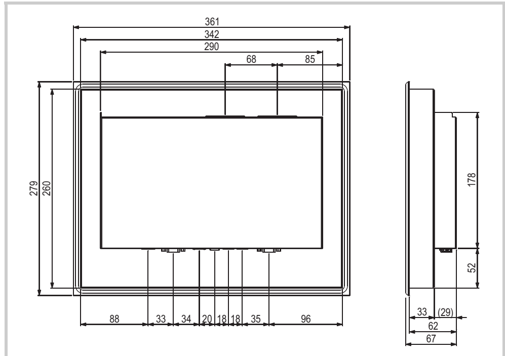
Abb. 31 Mechanical dimensions of the 12.1" devices in mm
