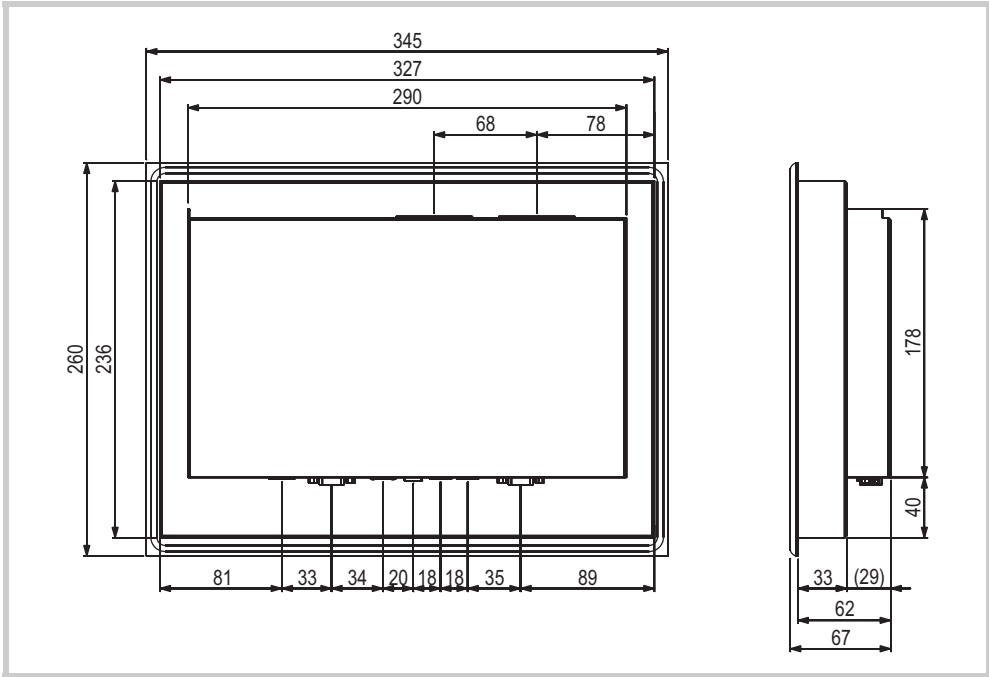
Abb. 30 Mechanical dimensions of the 10.4" devices in mm
