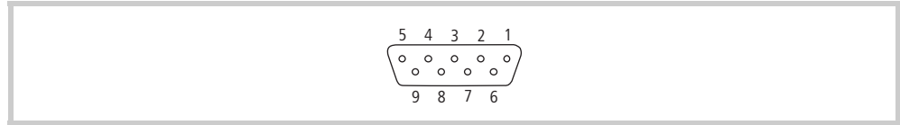
Abb. 17 Profibus interface (9-pin, D-Sub, female, UNC)
