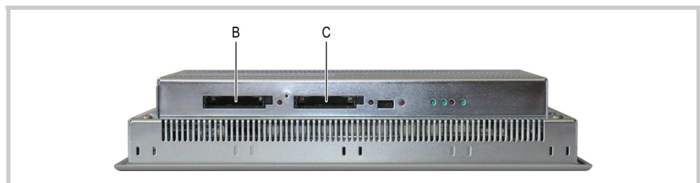
Abb. 29 Service side of the device (CF slot cover removed)
