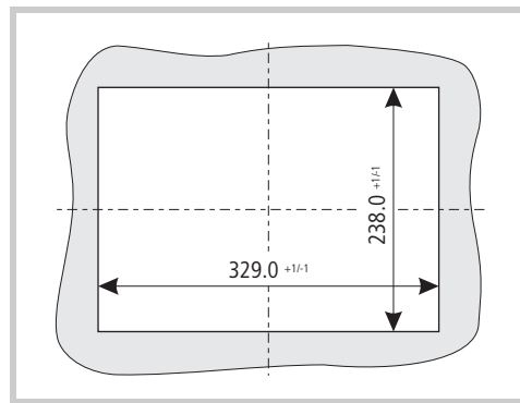
Abb. 19 Mounting cutout for 10.4" devices
