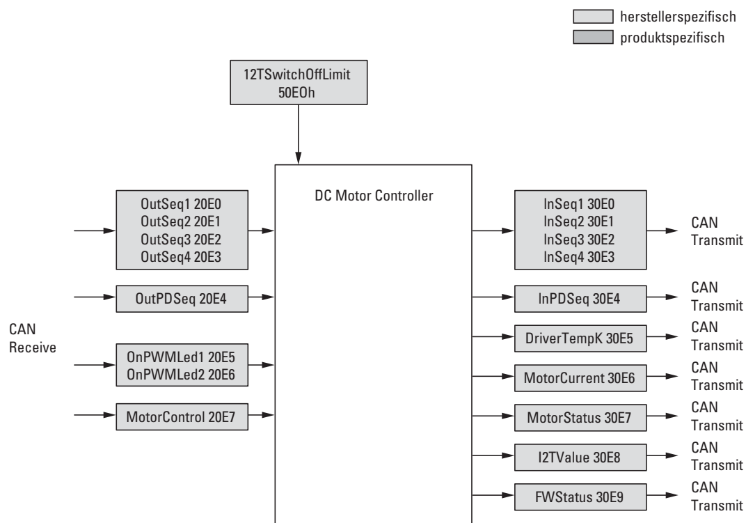
Figure 85: Block diagram showing the various CANopen objects
