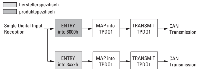
Figure 57: Block diagram showing the various CANopen objects for digital inputs
