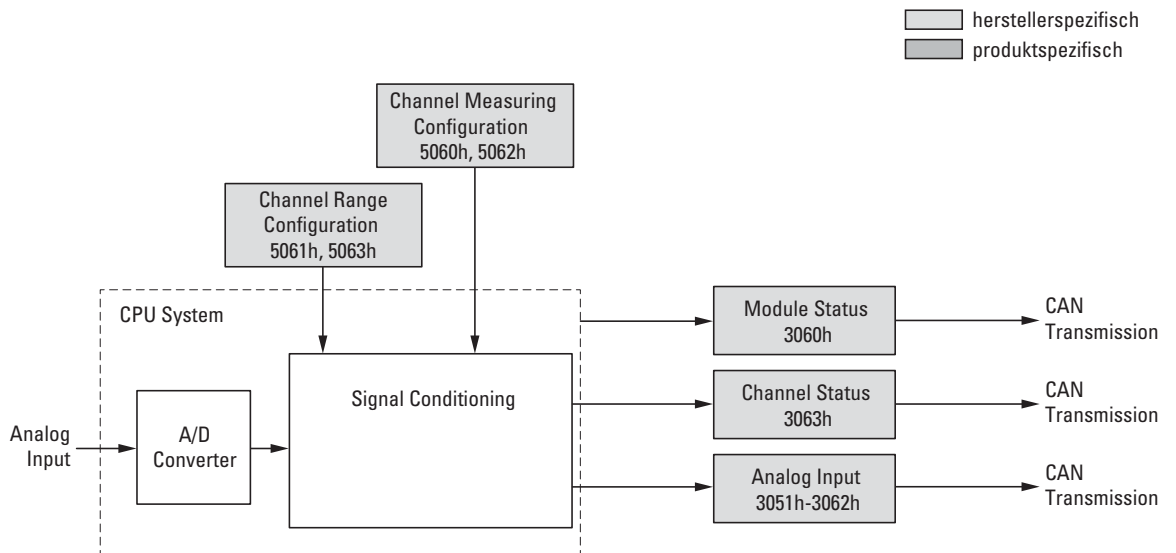
Figure 84: Block diagram showing the various CANopen objects
