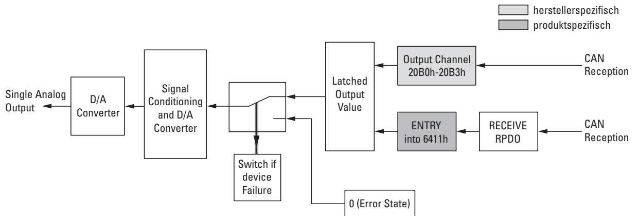
Figure 79: Block diagram showing the various CANopen objects for analog outputs
