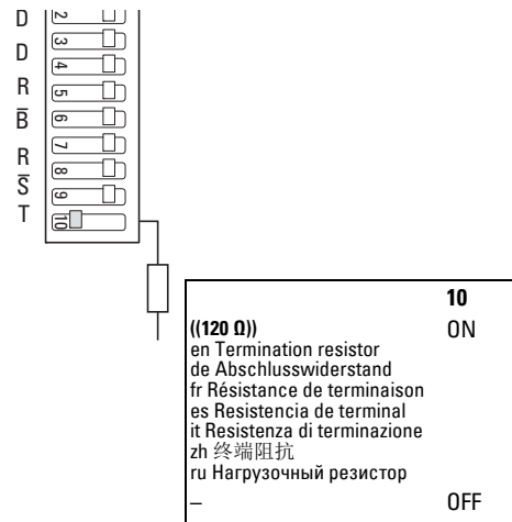
Figure 9: Activated bus termination resistor
