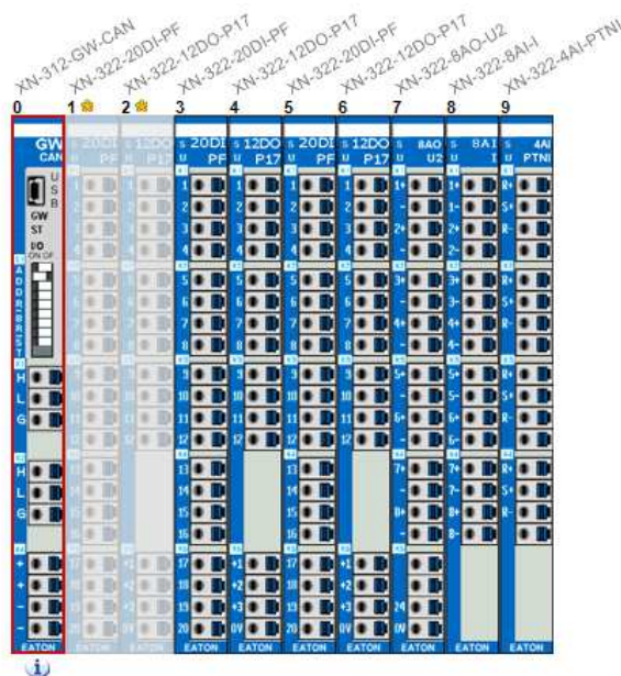
Figure 95: XN300-Assist with full configuration and reduced assembly
