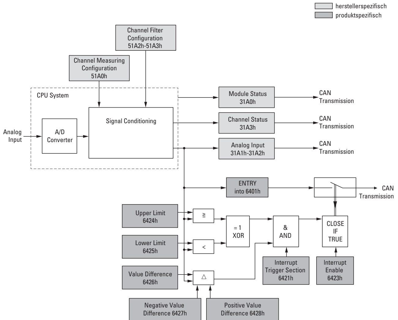
Figure 76: Block diagram showing the various CANopen objects for analog inputs
