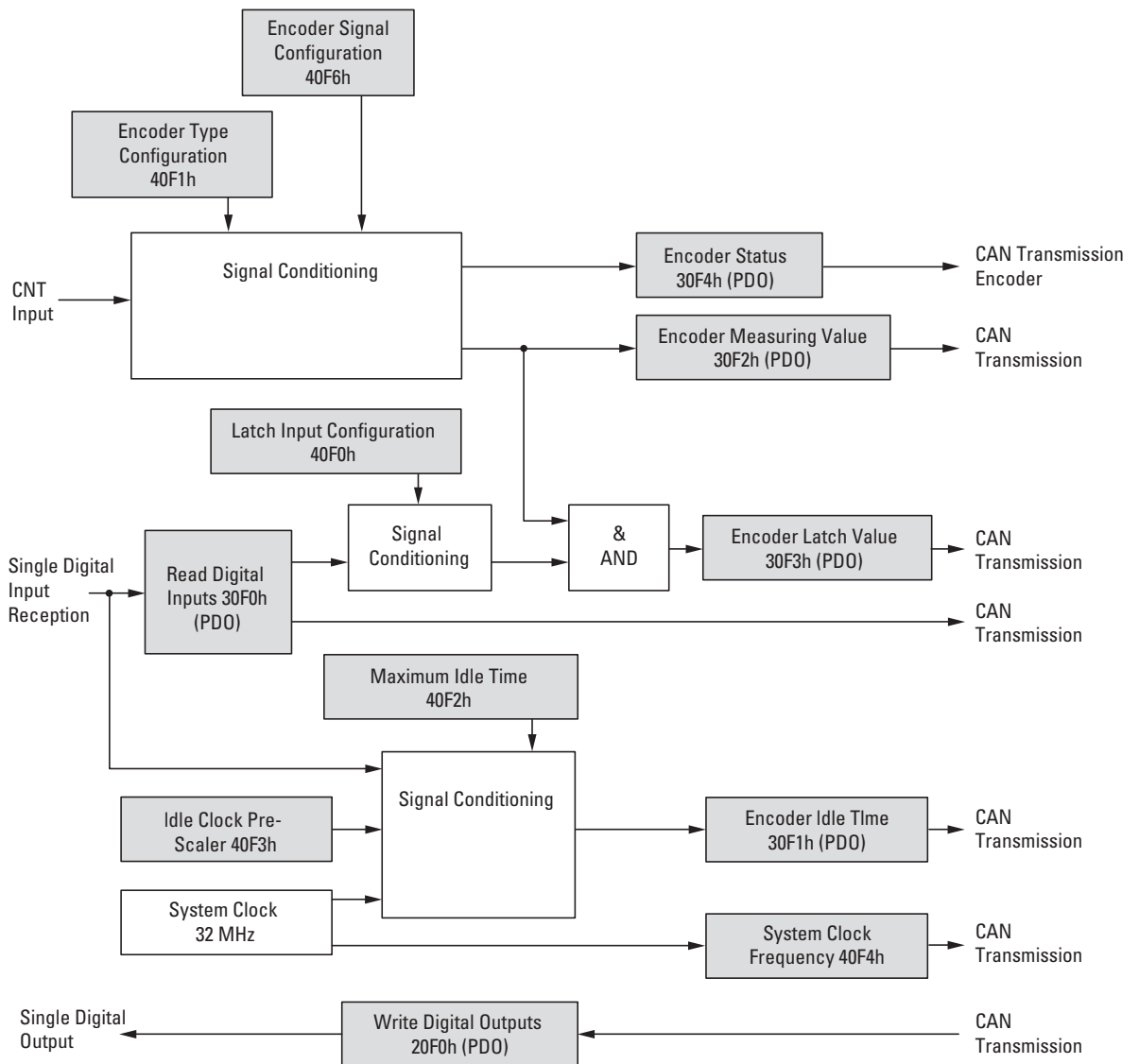
Figure 86: Block diagram showing the various CANopen objects for analog inputs
