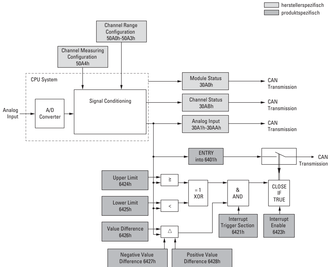
Figure 74: Block diagram showing the various CANopen objects
