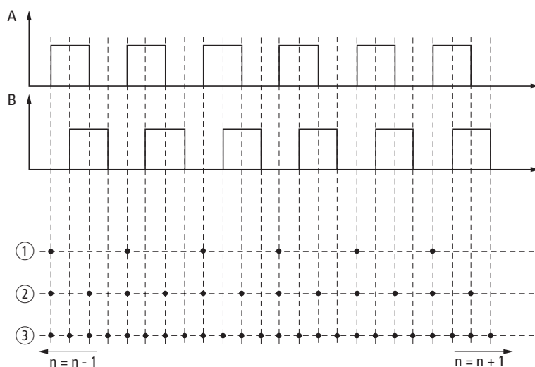
Figure 88: Signal diagram
