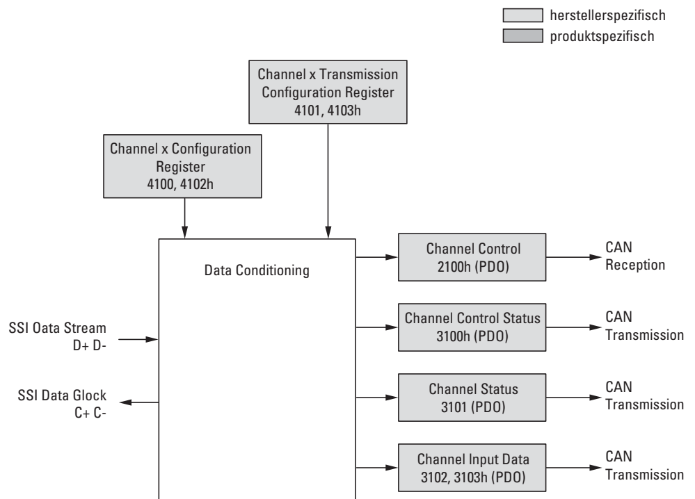
Figure 89: Block diagram showing the various CANopen objects for transmitting data streams
