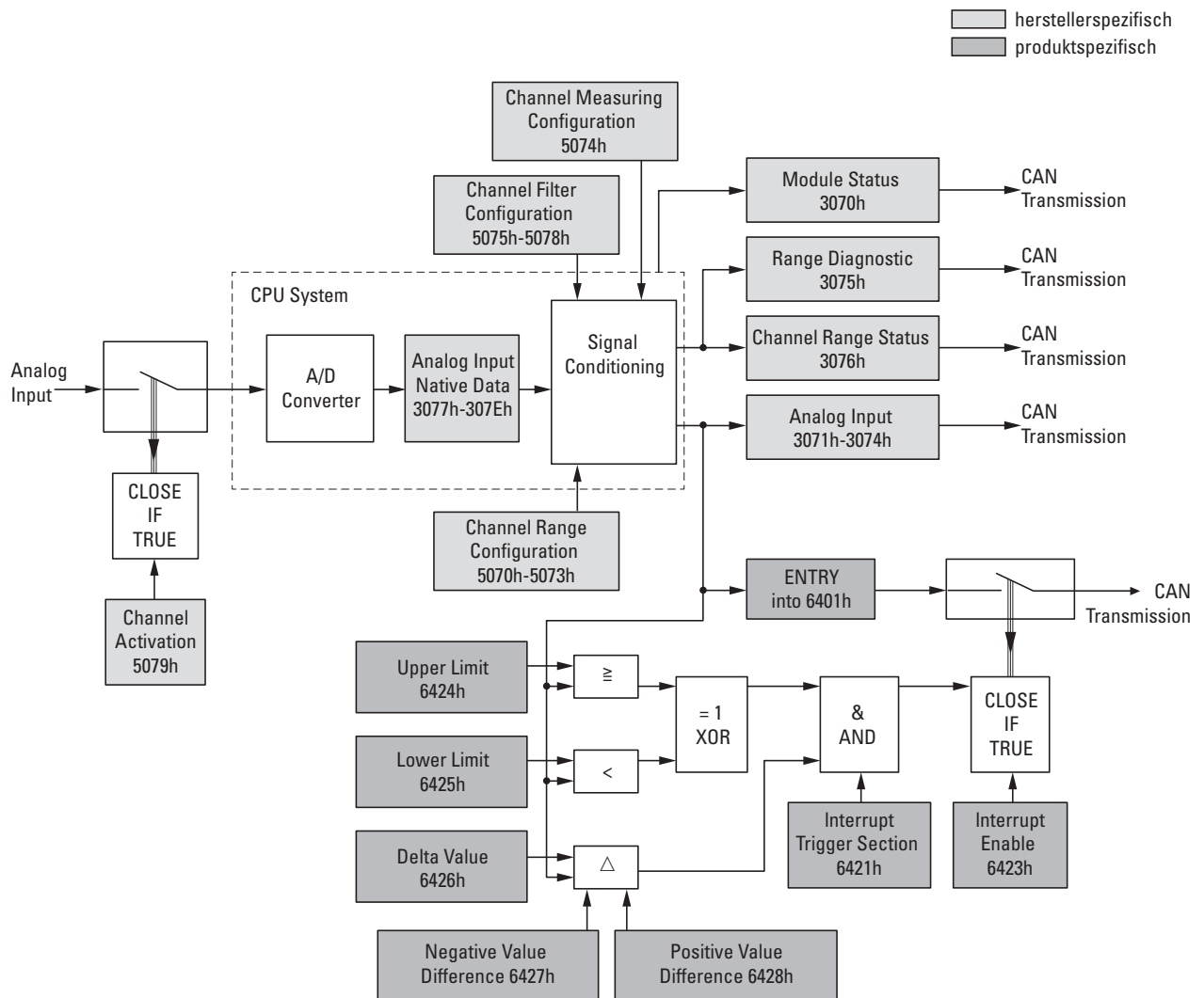
Figure 71: Block diagram showing the various CANopen objects for analog inputs
