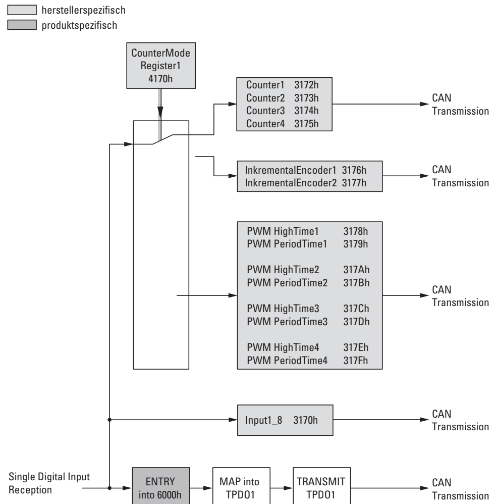
Figure 66: Block diagram showing the various CANopen objects for digital inputs
