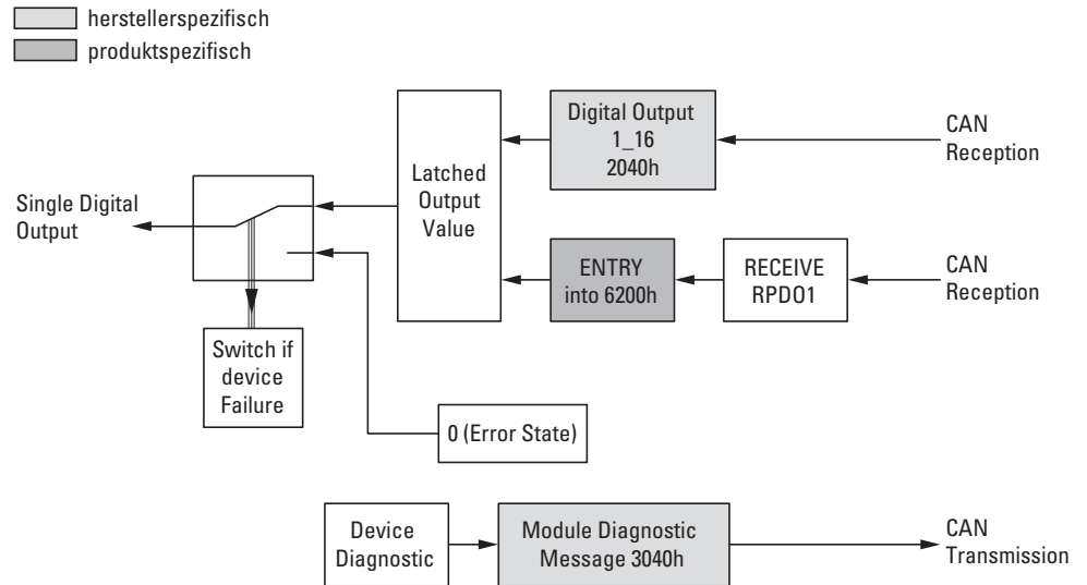
Figure 60: Block diagram showing the various CANopen objects for digital outputs
