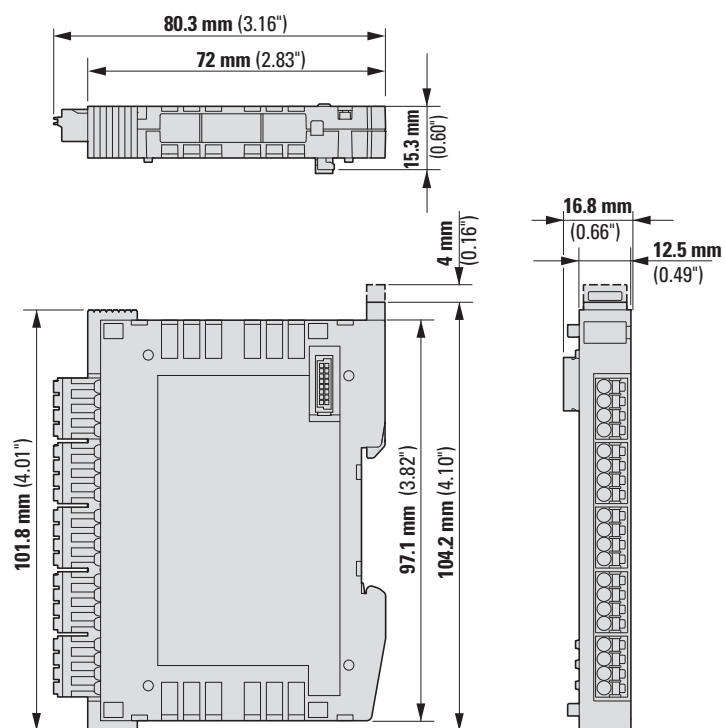
Figure 96: Dimensions XN-312-GW-CAN
