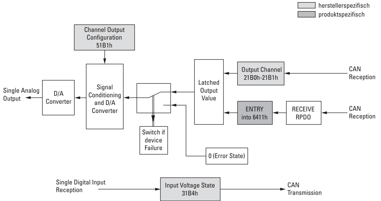
Figure 81: Block diagram showing the various CANopen objects for analog outputs
