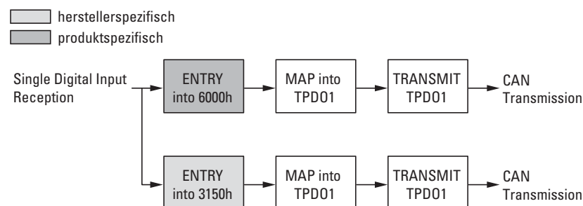
Figure 51: Block diagram showing the various CANopen objects for digital inputs
