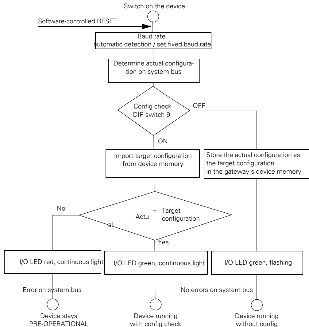
Figure 26: Switching on the device with and without a config check
