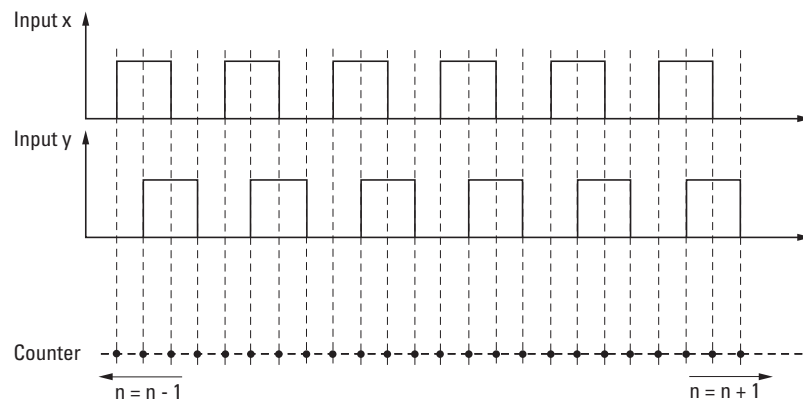
Figure 68: Timing diagram showing how inputs (x/y) = (1/2) or (3/4) of the incremental encoder register in the XN-322-16DIO-PC05 module count with X4 encoding
