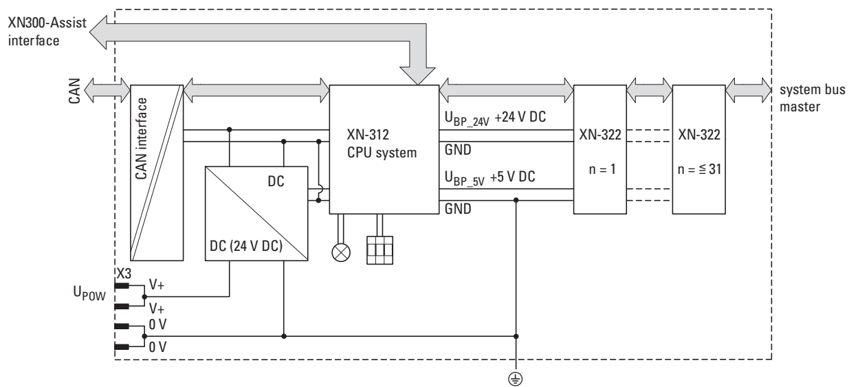
Figure 20: Functional diagram of XN300 system
