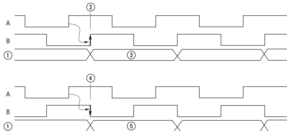
Figure 87: Signal diagram for signals A and B
