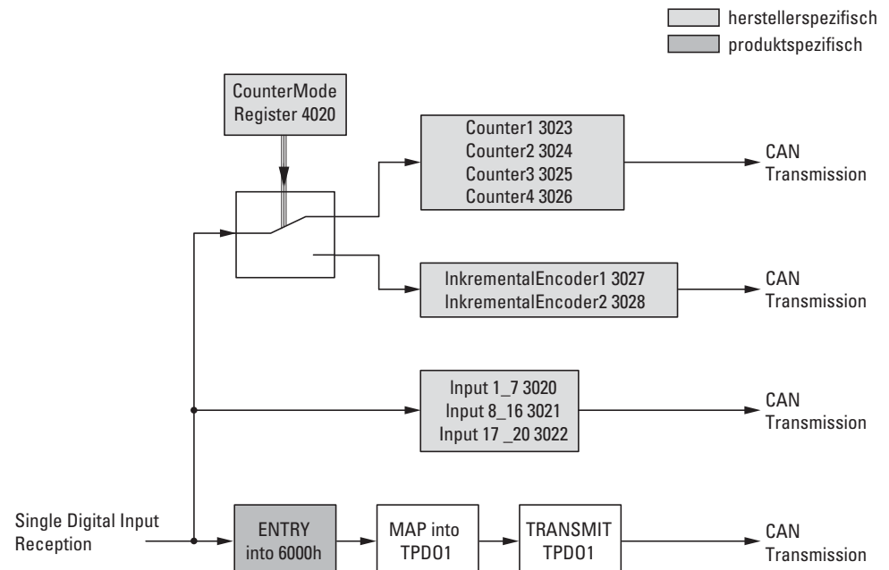
Figure 55: Block diagram showing the various CANopen objects for digital inputs
