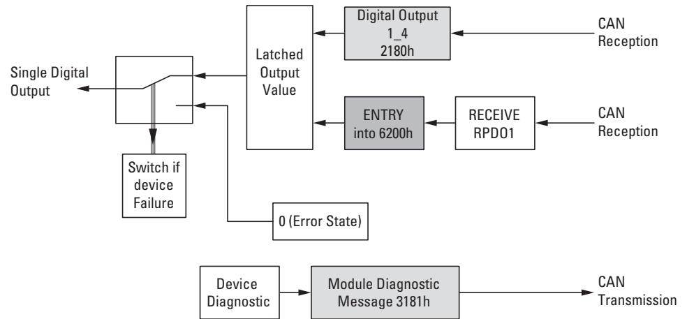
Figure 63: Block diagram showing the various CANopen objects for digital outputs
