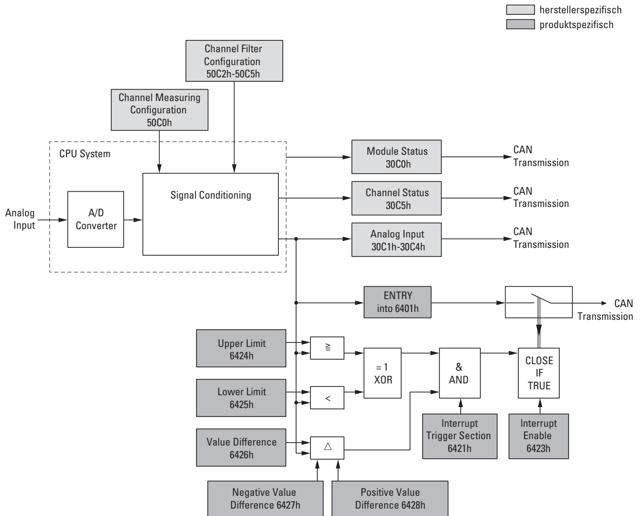
Figure 82: Block diagram showing the various CANopen objects for analog inputs
