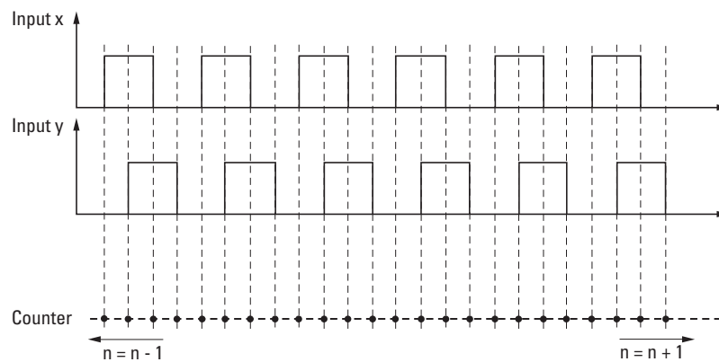
Figure 56: Timing diagram showing how the inputs of the incremental encoder register in the XN-322-20DI-PCNT module count with X4 encoding
