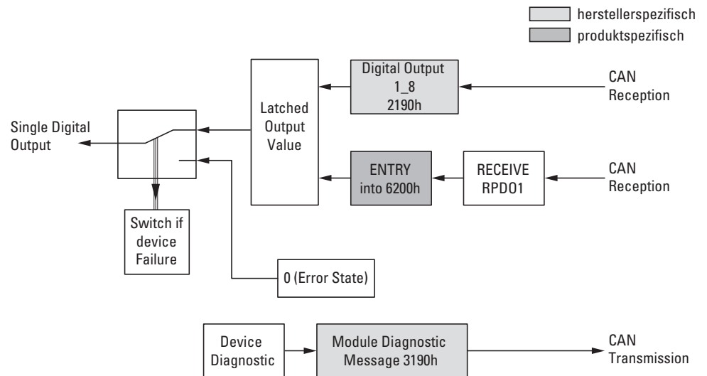
Figure 59: Block diagram showing the various CANopen objects for digital outputs
