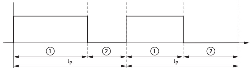
Figure 69: PWM signal measurement
