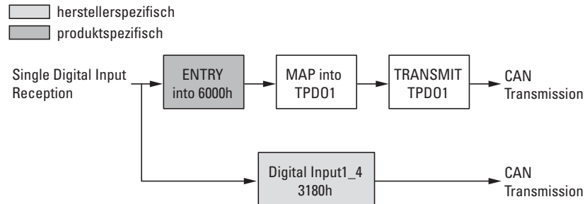
Figure 62: Block diagram showing the various CANopen objects for digital inputs
