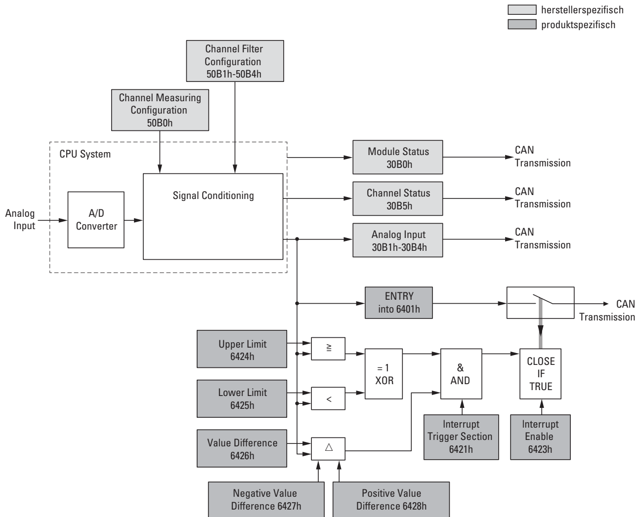
Figure 78: Block diagram showing the various CANopen objects for analog inputs
