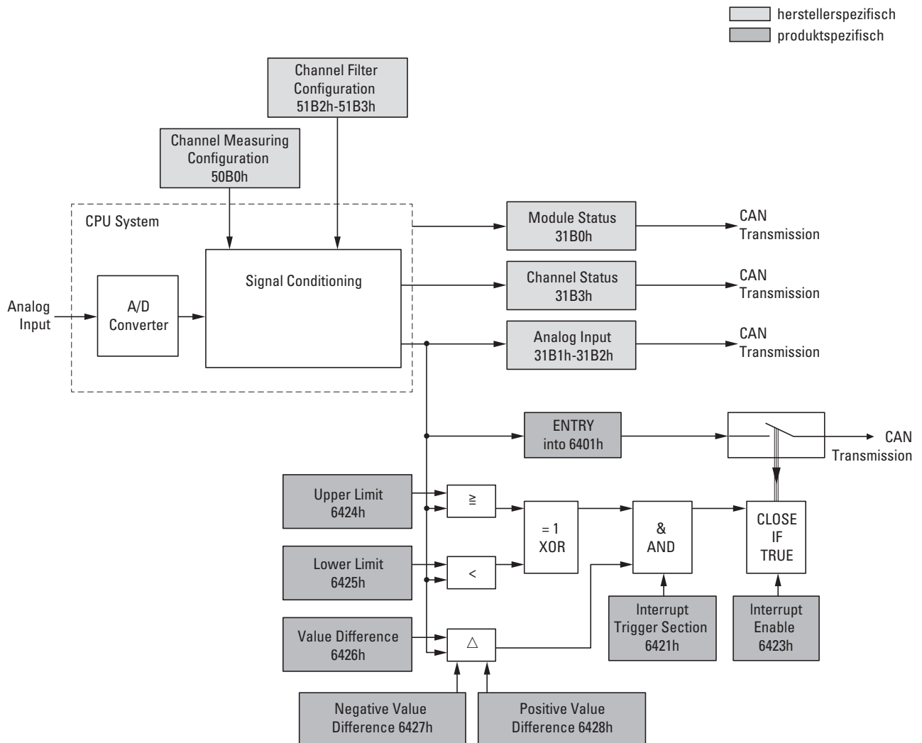
Figure 80: Block diagram showing the various CANopen objects for analog inputs
