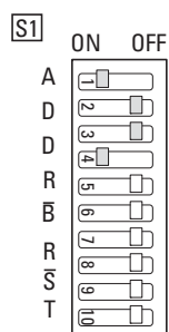
Figure 8: Example: Setting field bus address 18_{dec} on the gateway
