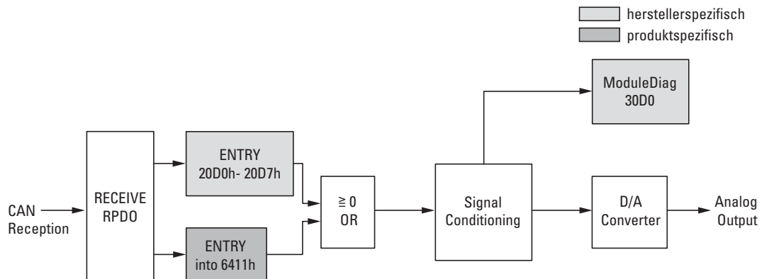
Figure 75: Block diagram showing the various CANopen objects for analog outputs
