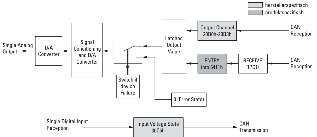
Figure 83: Block diagram showing the various CANopen objects for analog outputs
