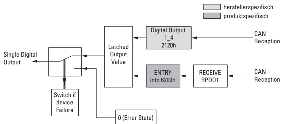
Figure 58: Block diagram showing the various CANopen objects for digital outputs
