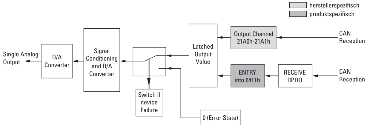
Figure 77: Block diagram showing the various CANopen objects for analog outputs
