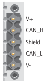
Abbildung 7: Open Style Connector (male)
