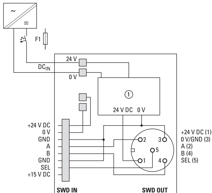
SWD4-SFL8-12
