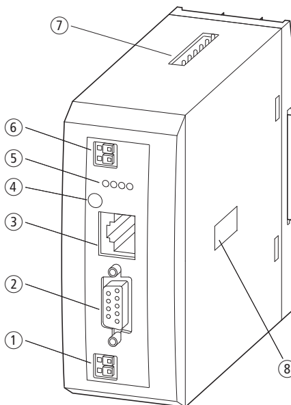
Figura 1: Vista frontale EU5C-SWD-DP
