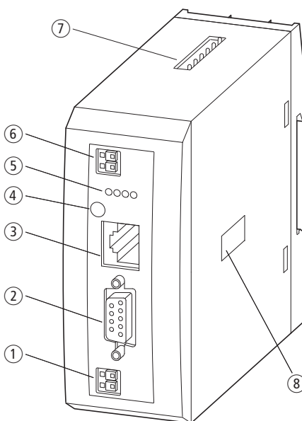
Figura 28: Vista frontale EU5C-SWD-CAN
