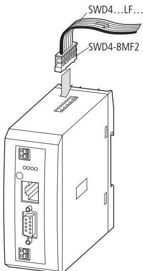
Figura 6: Collegamento SmartWire-Darwin
