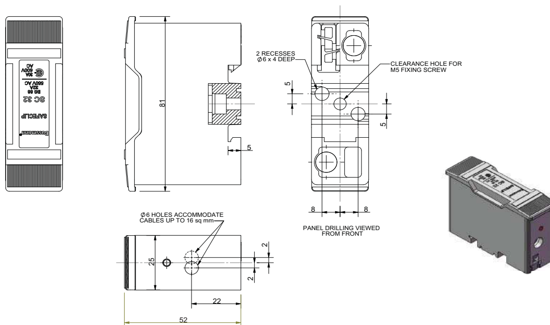
SC32H-D 32 A, Front connected
