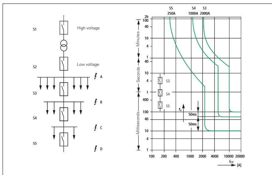
Figure 4: Example of a cascade type network design. The switches on the various network levels should shutdown selectively. This can be implemented with time selectivity. The switch on the lowest level (S 5 in the example) features a non-delayed short-circuit release, all upstream switches have a short-delay time of about 50 ms, 100 ms etc.
