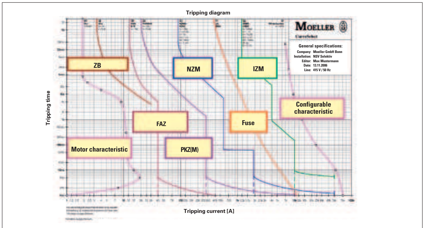
Figure 1: Representation of the tripping characteristic of different protective devices on the same time and current scale. The device data and settings are stated at the upper end of the curves.
