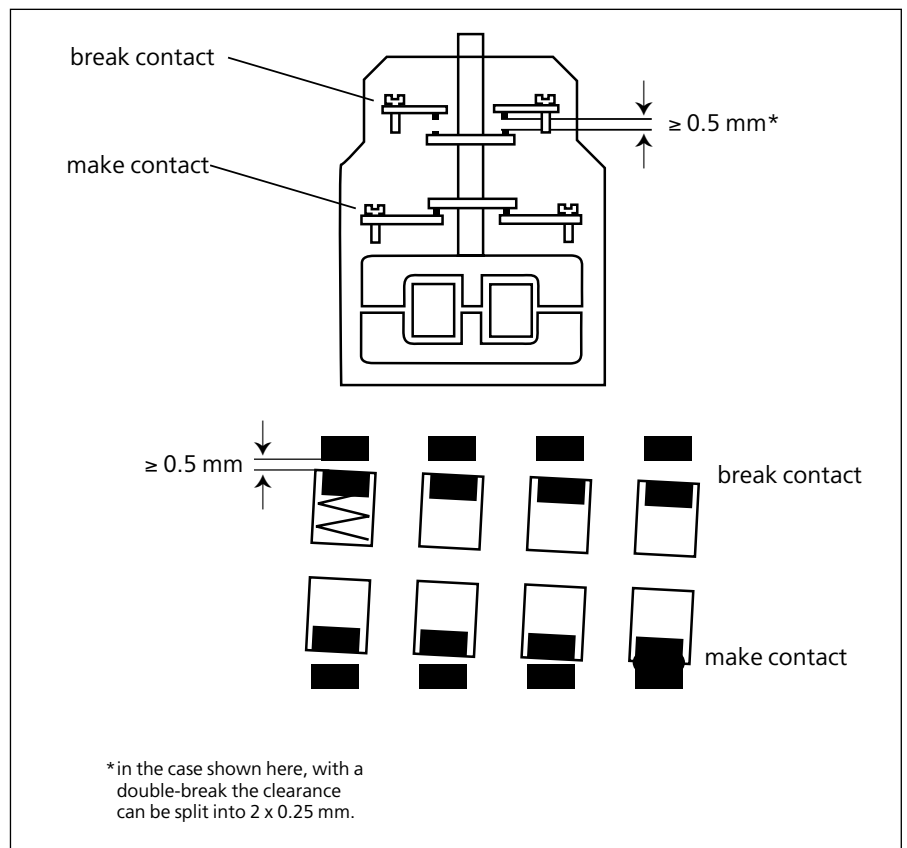
Figure 2: If for example the outer right make contact welds on a contactor, the contact bridge of the switched off contactor may skew. With "positively-driven contacts" it is required that the break contact does not close in this case, but rather, that a clearance of 0.5 mm is retained between the contacts for the entire lifespan of the contactor. Various safety circuits are based on the assumption that the break contact and make contact of a contactor can never close simultaneously.
