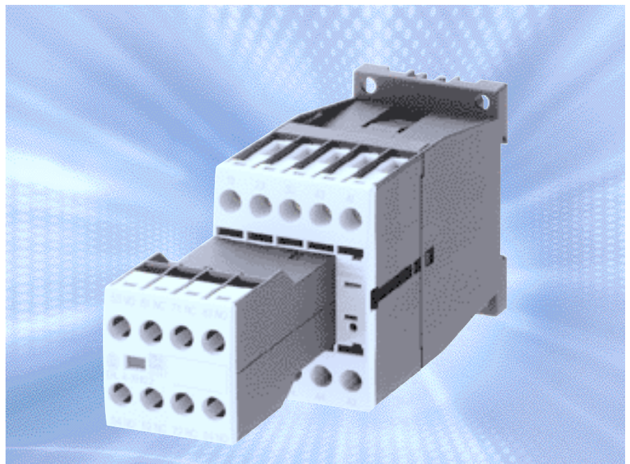
Figure 1: The contactor relay from the new Moeller xStart range features 4 auxiliary contacts in the basic unit. Today, it is generally the case that further contacts (2 or 4 here) are added on an application-specific basis, based on the use of a modular system.
