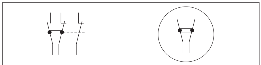
Figure 4: Left: Example of a standard compliant representation of positively driven N/O and N/C contacts and a non positively driven N/C contact in a circuit diagram. Right: Example of a possible marking on a device, for devices which also contain positively driven contacts.
