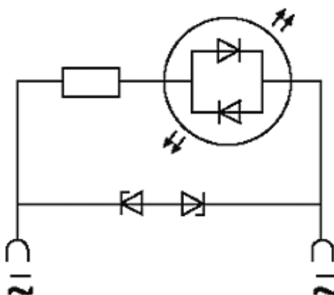
LED + Zenerdiode
