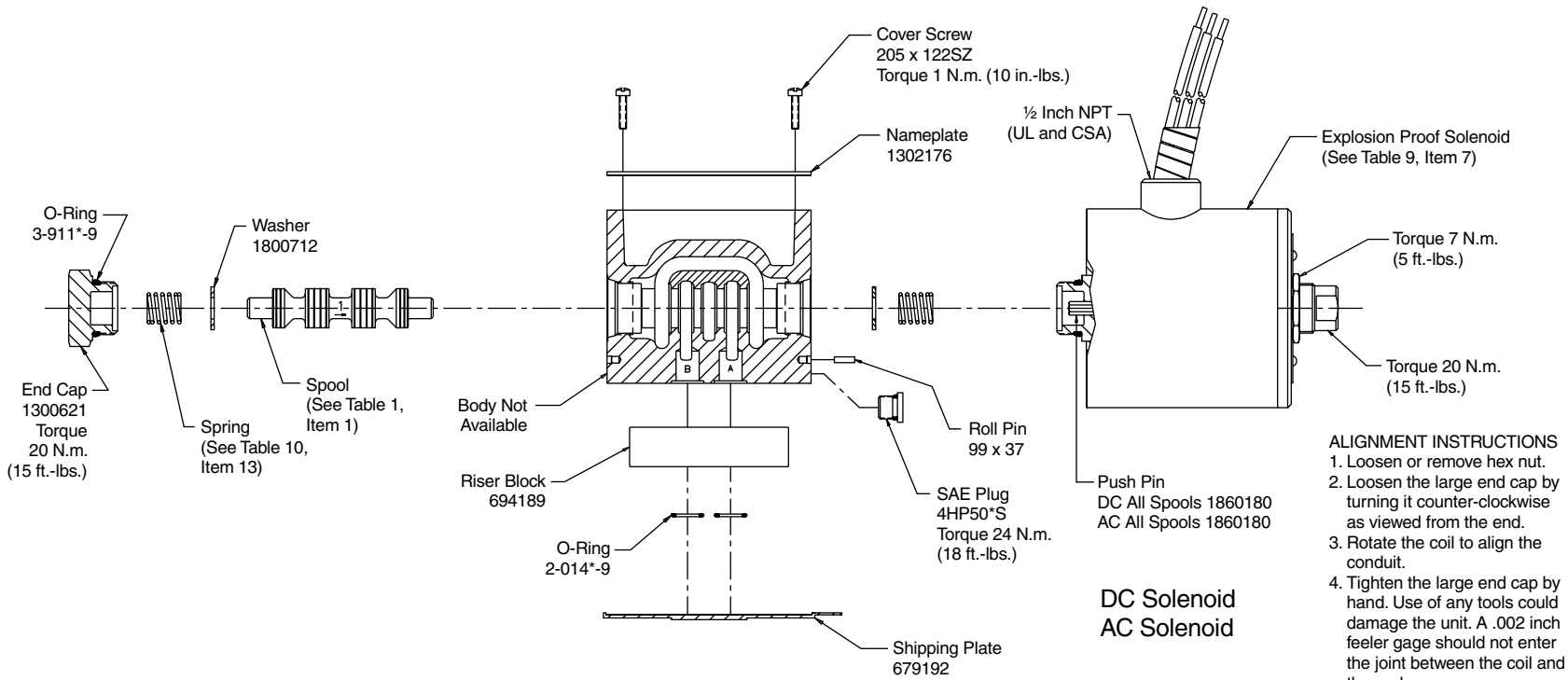
D3W Single AC Solenoid Model D3W Single DC Solenoid Model
