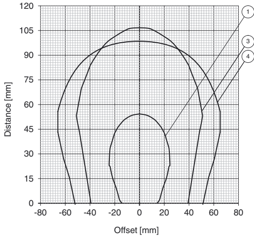
Reading range in air IQC22-39
