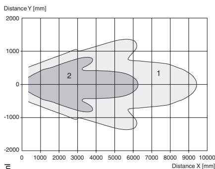
Distance Y [mm] 2000 1000 0 -1000 -2000 0 1000 2000 3000 4000 5000 6000 7000 8000 9000 10000 Distance X [mm] Y X Curve 1: flat surface 100 mm x 100 mm Curve 2: round bar, Ø 25 mm
