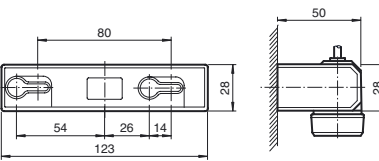
Mounting dimensions for swivel
