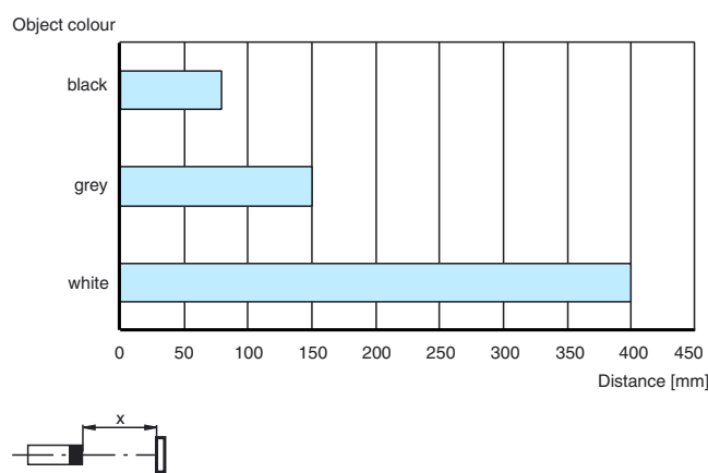
Detection ranges VT18-8-400
