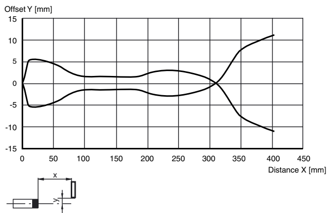
Characteristic response curve VT18-8-400
