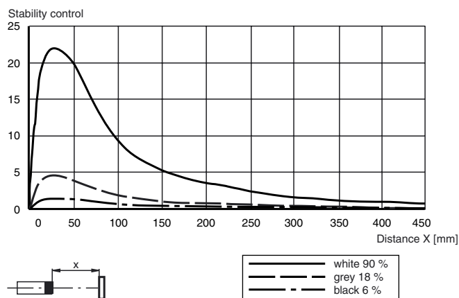
Relative received light strength VT18-8-400
